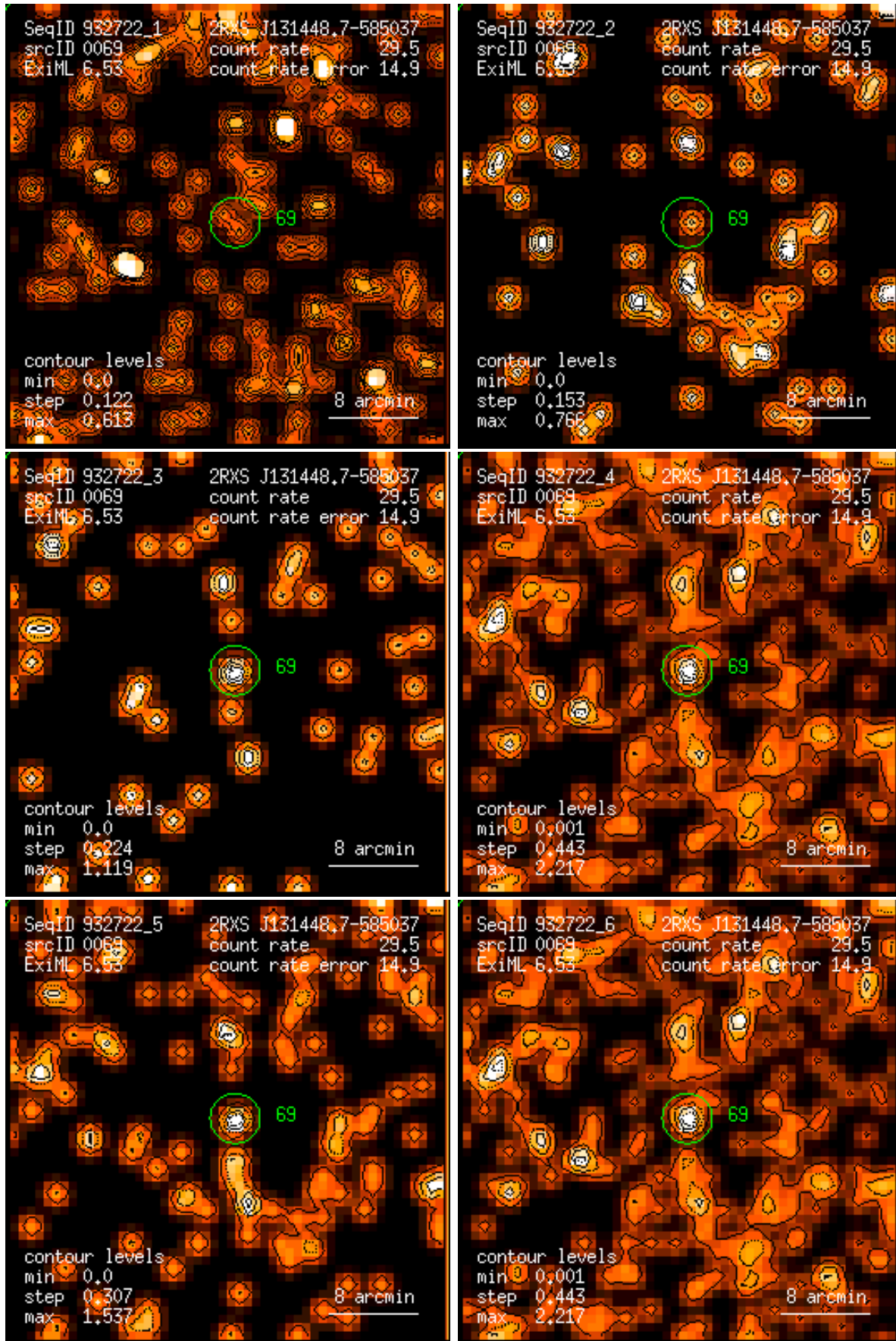
Figure 69: RASS 932722: detection 0069: band rate images, Gaussian filter: (1) PSPC channels 11 – 41, (2) 52 – 90, (3) 91 – 201, (4) 11 – 235, (5) 52 – 201, (6) 11 – 201. Broad band rates in counts/ks. Band rate contour levels in counts/ks/arcmin 2 .
