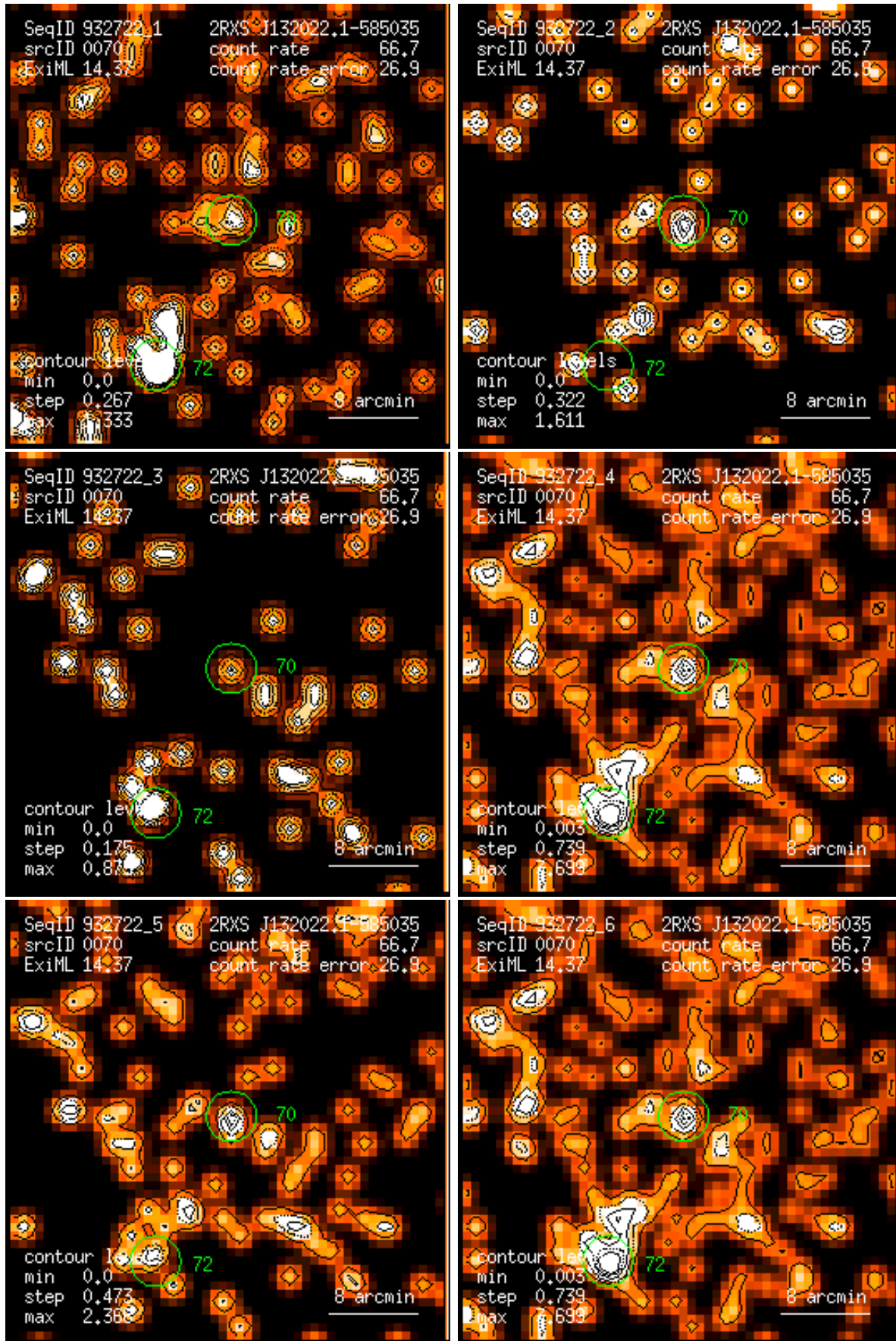
Figure 70: RASS 932722: detection 0070: band rate images, Gaussian filter: (1) PSPC channels 11 – 41, (2) 52 – 90, (3) 91 – 201, (4) 11 – 235, (5) 52 – 201, (6) 11 – 201. Broad band rates in counts/ks. Band rate contour levels in counts/ks/arcmin 2 .
