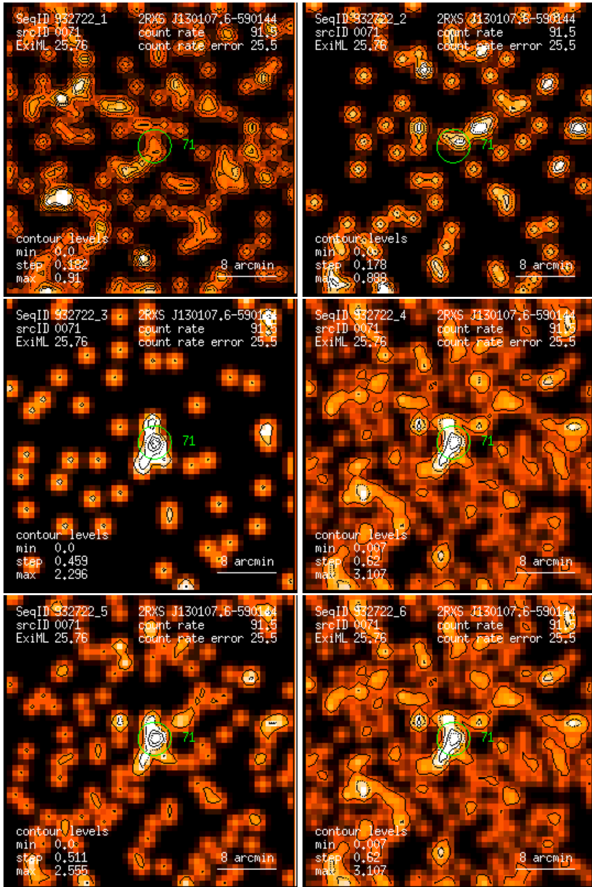
Figure 71: RASS 932722: detection 0071: band rate images, Gaussian filter: (1) PSPC channels 11 – 41, (2) 52 – 90, (3) 91 – 201, (4) 11 – 235, (5) 52 – 201, (6) 11 – 201. Broad band rates in counts/ks. Band rate contour levels in counts/ks/arcmin 2 .
