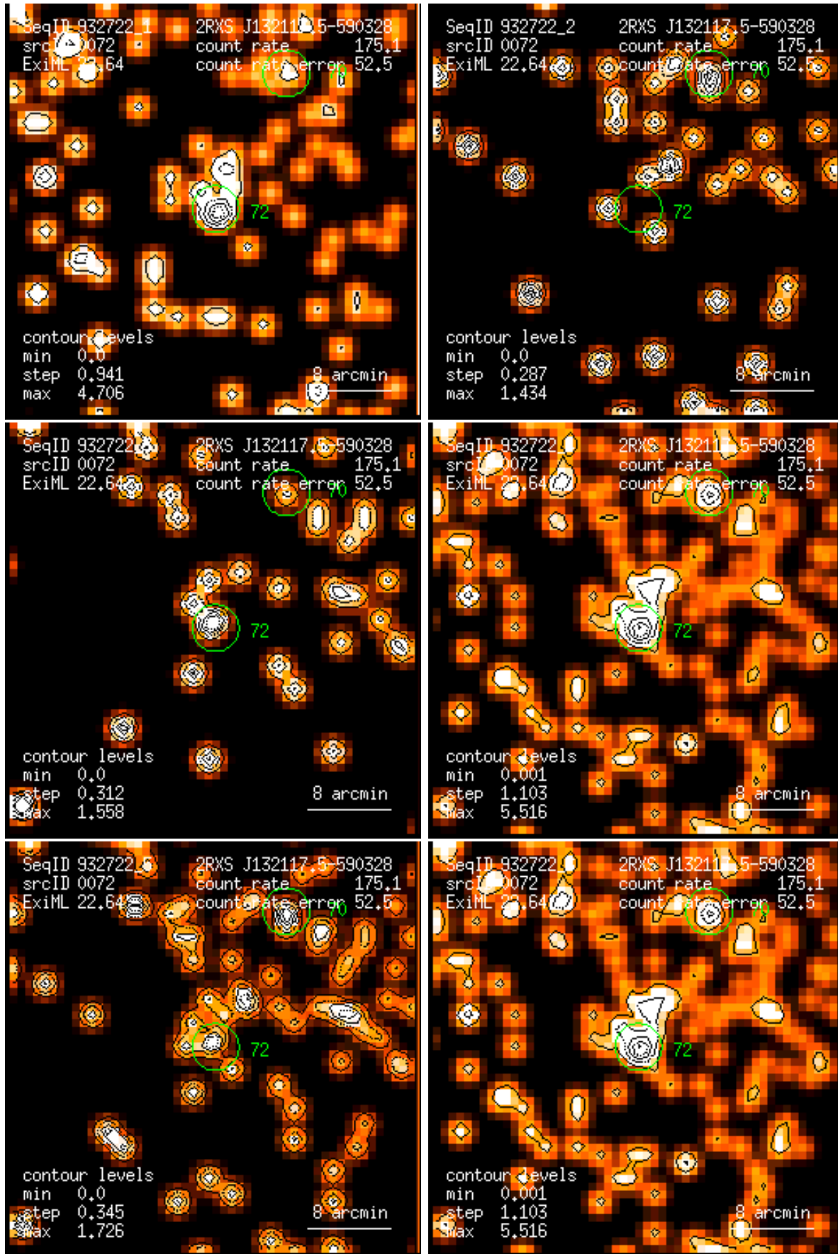
Figure 72: RASS 932722: detection 0072: band rate images, Gaussian filter: (1) PSPC channels 11 – 41, (2) 52 – 90, (3) 91 – 201, (4) 11 – 235, (5) 52 – 201, (6) 11 – 201. Broad band rates in counts/ks. Band rate contour levels in counts/ks/arcmin 2 .
