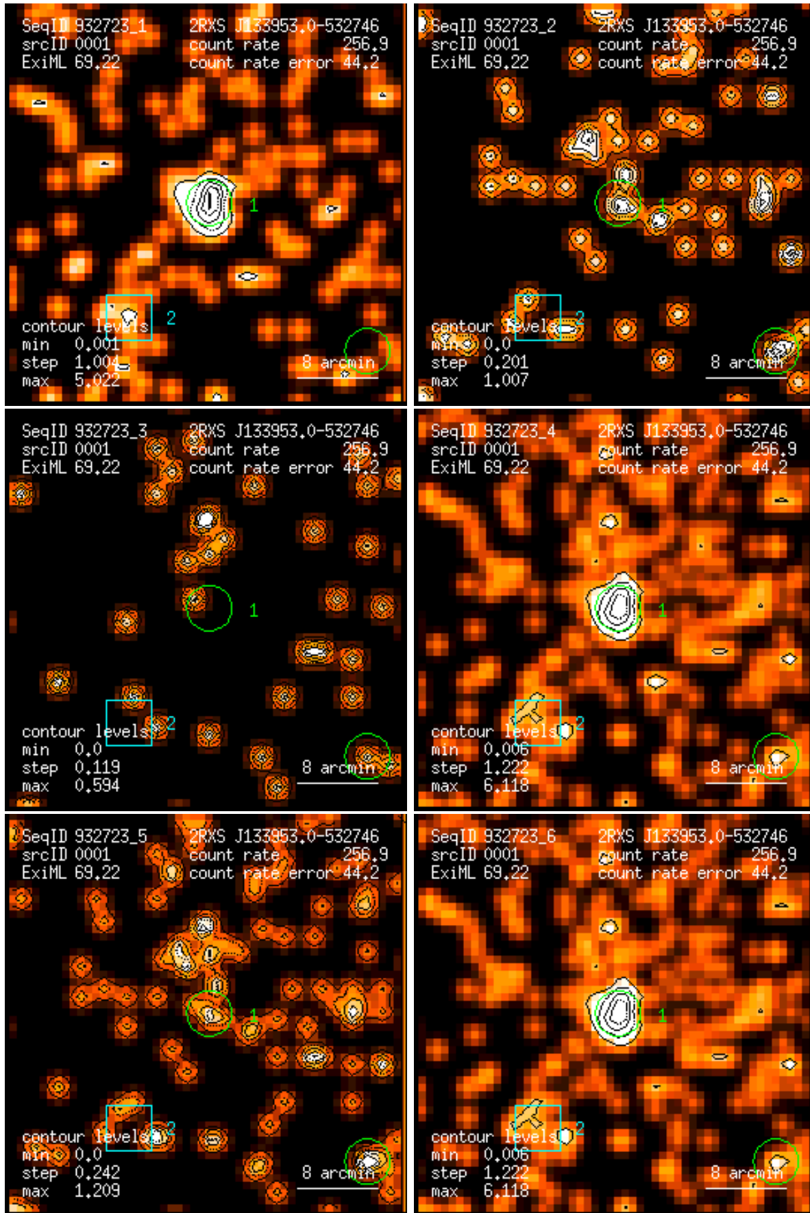
Figure 1: RASS 932723: detection 0001: band rate images, Gaussian filter: (1) PSPC channels 11 – 41, (2) 52 – 90, (3) 91 – 201, (4) 11 – 235, (5) 52 – 201, (6) 11 – 201. Broad band rates in counts/ks. Band rate contour levels in counts/ks/arcmin 2 .
