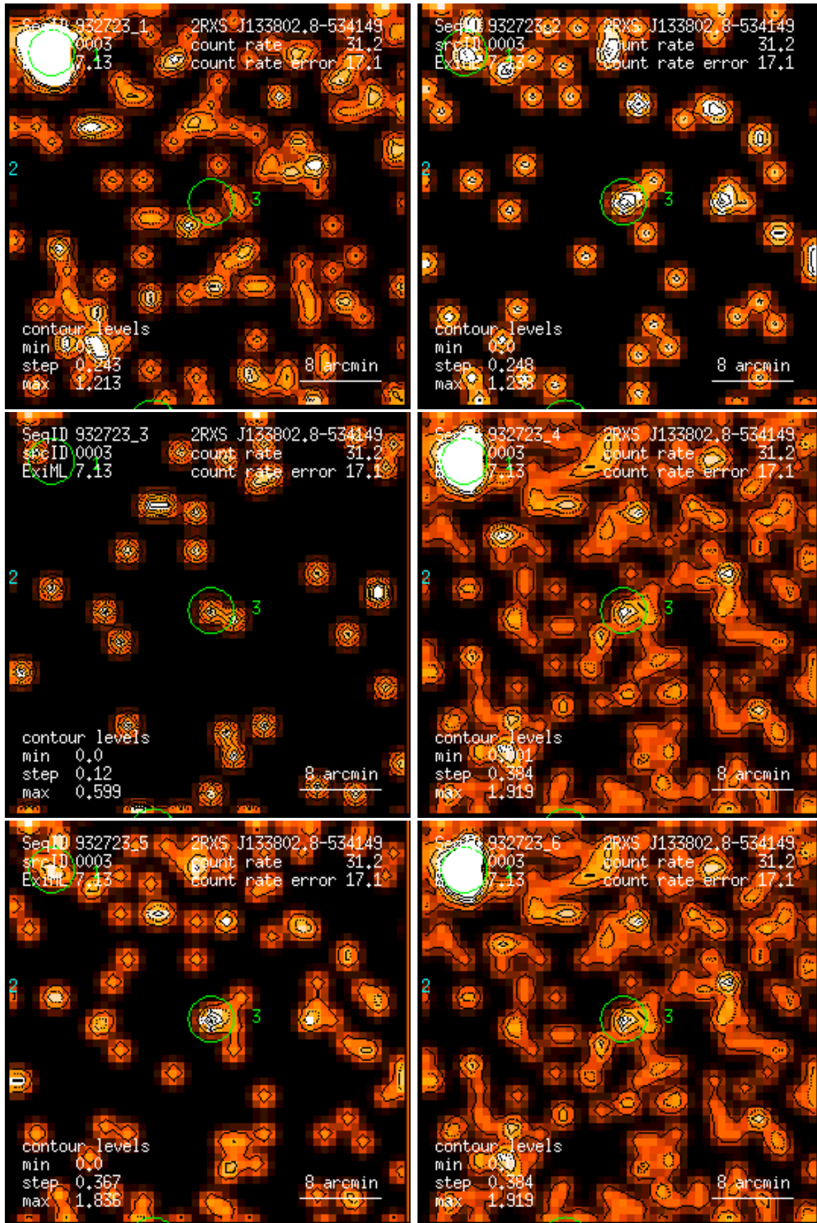
Figure 3: RASS 932723: detection 0003: band rate images, Gaussian filter: (1) PSPC channels 11 – 41, (2) 52 – 90, (3) 91 – 201, (4) 11 – 235, (5) 52 – 201, (6) 11 – 201. Broad band rates in counts/ks. Band rate contour levels in counts/ks/arcmin 2 .
