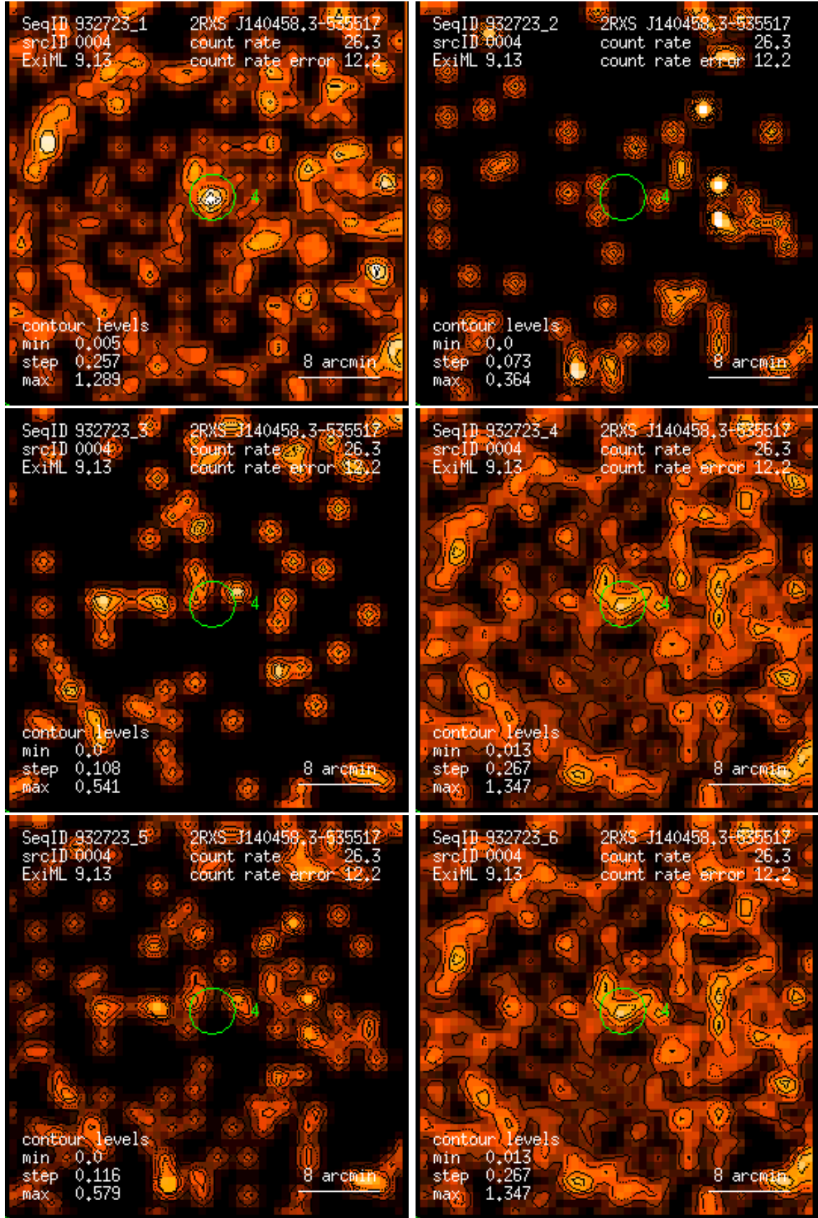
Figure 4: RASS 932723: detection 0004: band rate images, Gaussian filter: (1) PSPC channels 11 – 41, (2) 52 – 90, (3) 91 – 201, (4) 11 – 235, (5) 52 – 201, (6) 11 – 201. Broad band rates in counts/ks. Band rate contour levels in counts/ks/arcmin 2 .
