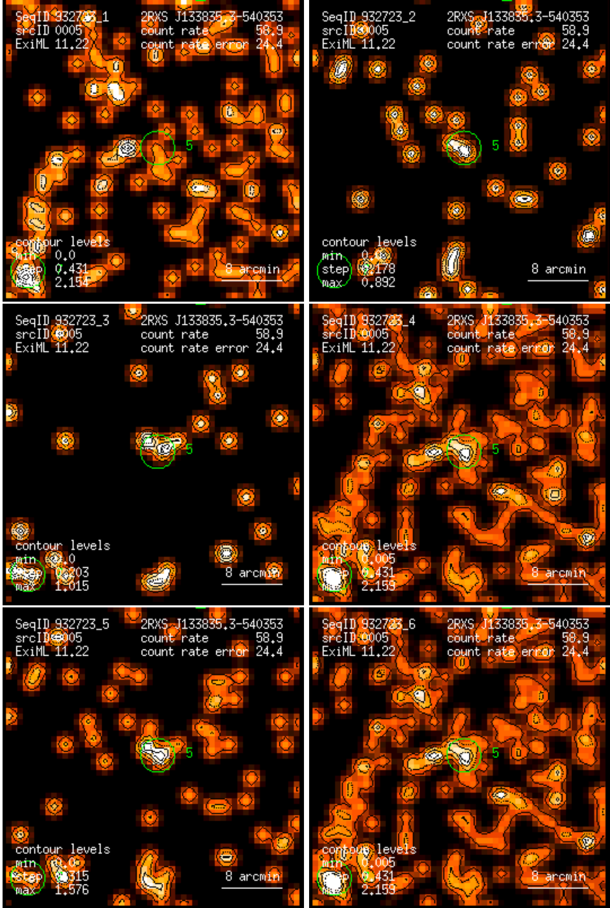
Figure 5: RASS 932723: detection 0005: band rate images, Gaussian filter: (1) PSPC channels 11 – 41, (2) 52 – 90, (3) 91 – 201, (4) 11 – 235, (5) 52 – 201, (6) 11 – 201. Broad band rates in counts/ks. Band rate contour levels in counts/ks/arcmin 2 .
