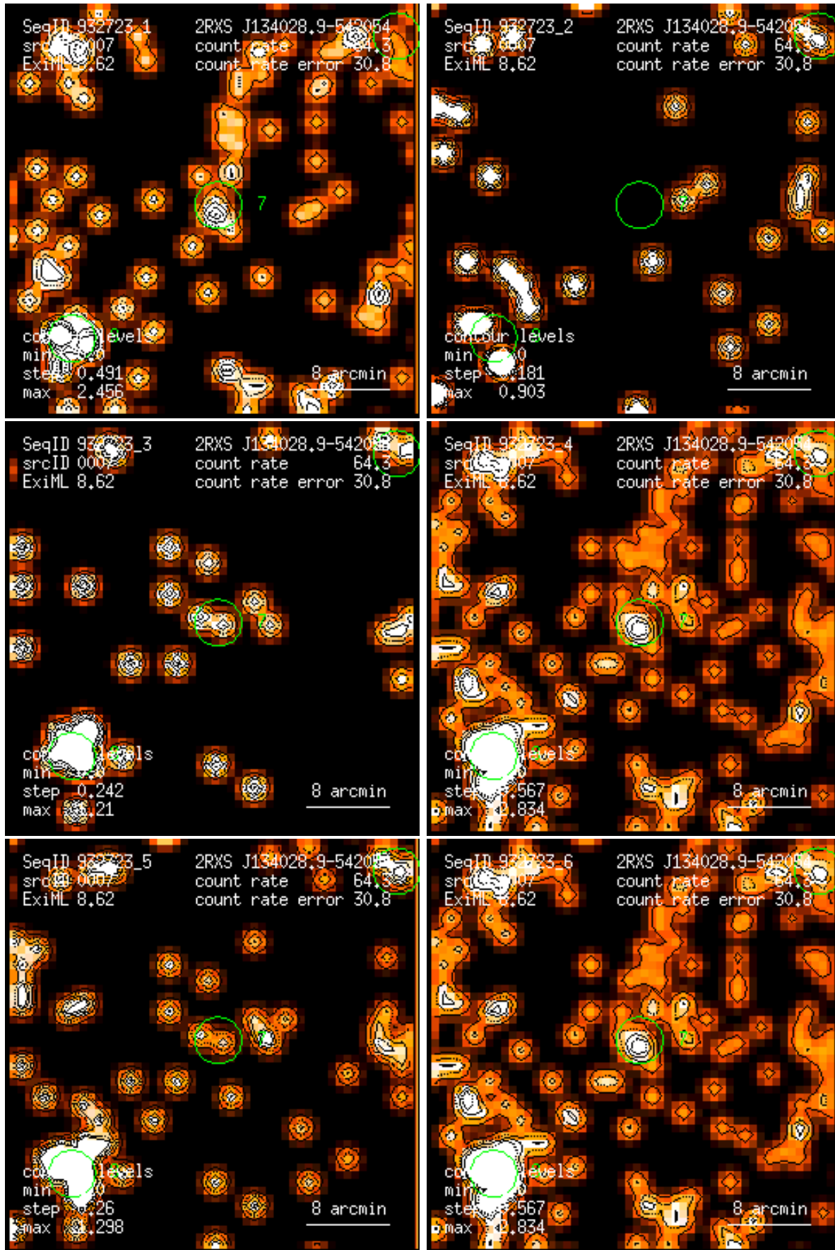
Figure 7: RASS 932723: detection 0007: band rate images, Gaussian filter: (1) PSPC channels 11 – 41, (2) 52 – 90, (3) 91 – 201, (4) 11 – 235, (5) 52 – 201, (6) 11 – 201. Broad band rates in counts/ks. Band rate contour levels in counts/ks/arcmin 2 .
