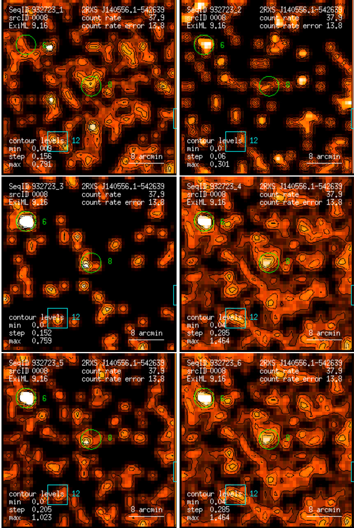
Figure 8: RASS 932723: detection 0008: band rate images, Gaussian filter: (1) PSPC channels 11 – 41, (2) 52 – 90, (3) 91 – 201, (4) 11 – 235, (5) 52 – 201, (6) 11 – 201. Broad band rates in counts/ks. Band rate contour levels in counts/ks/arcmin 2 .
