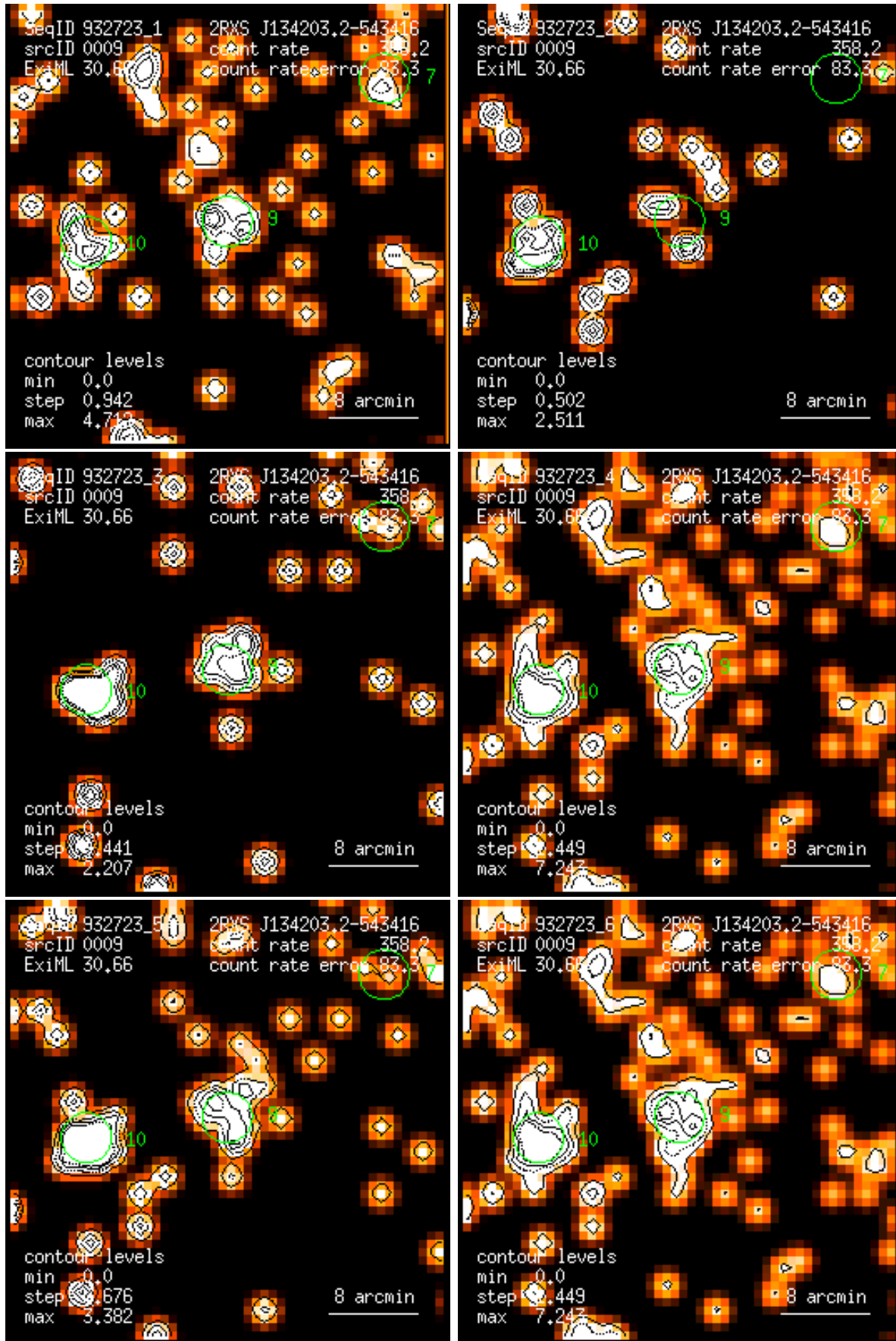
Figure 9: RASS 932723: detection 0009: band rate images, Gaussian filter: (1) PSPC channels 11 – 41, (2) 52 – 90, (3) 91 – 201, (4) 11 – 235, (5) 52 – 201, (6) 11 – 201. Broad band rates in counts/ks. Band rate contour levels in counts/ks/arcmin 2 .
