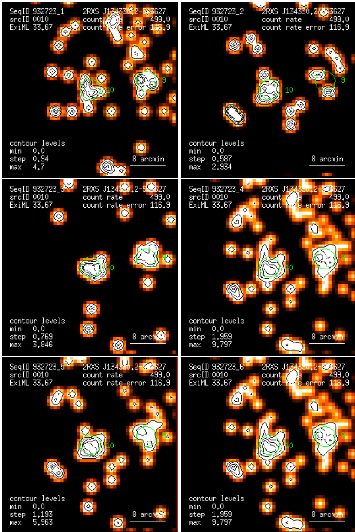
Figure 10: RASS 932723: detection 0010: band rate images, Gaussian filter: (1) PSPC channels 11 – 41, (2) 52 – 90, (3) 91 – 201, (4) 11 – 235, (5) 52 – 201, (6) 11 – 201. Broad band rates in counts/ks. Band rate contour levels in counts/ks/arcmin 2 .
