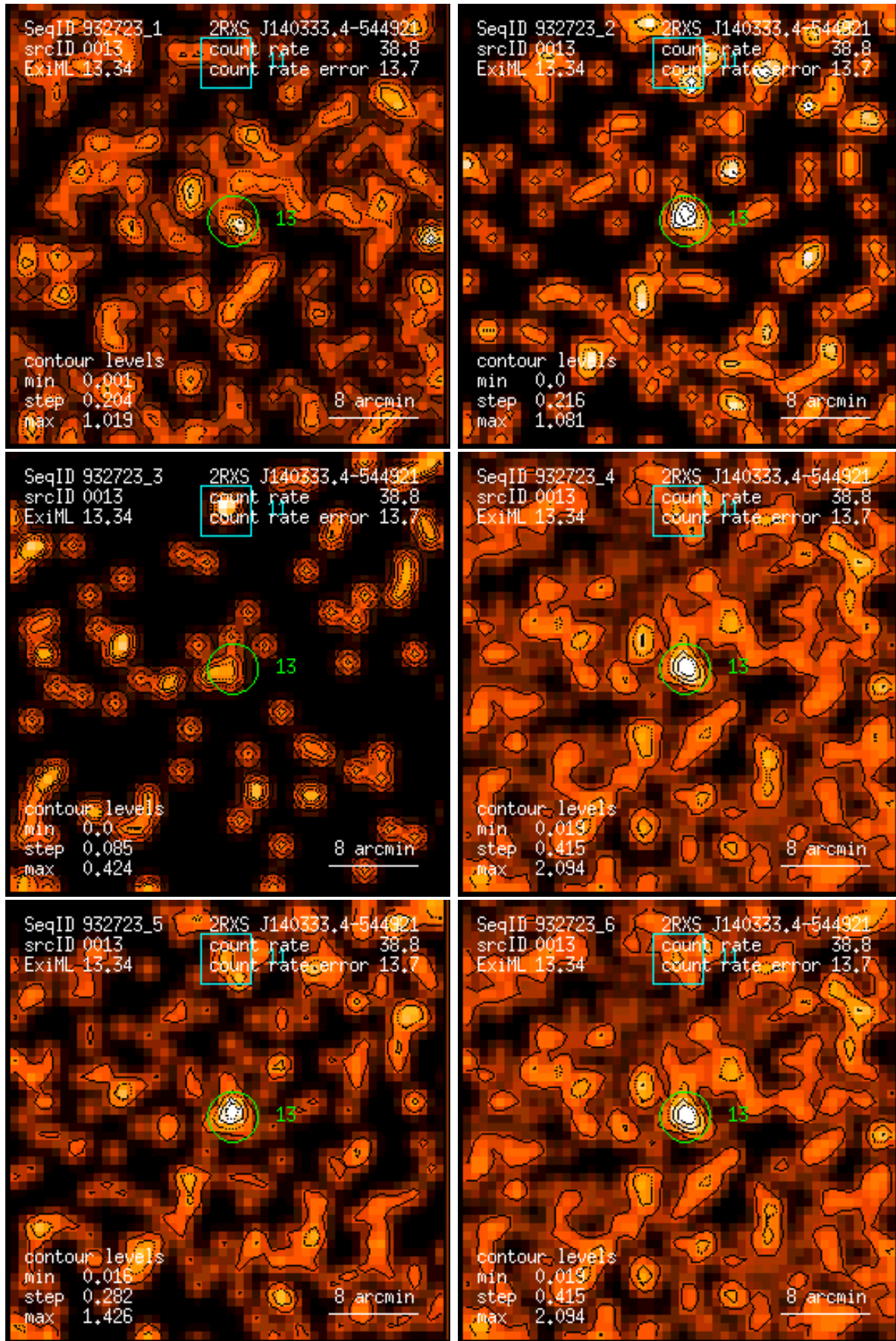
Figure 13: RASS 932723: detection 0013: band rate images, Gaussian filter: (1) PSPC channels 11 – 41, (2) 52 – 90, (3) 91 – 201, (4) 11 – 235, (5) 52 – 201, (6) 11 – 201. Broad band rates in counts/ks. Band rate contour levels in counts/ks/arcmin 2 .
