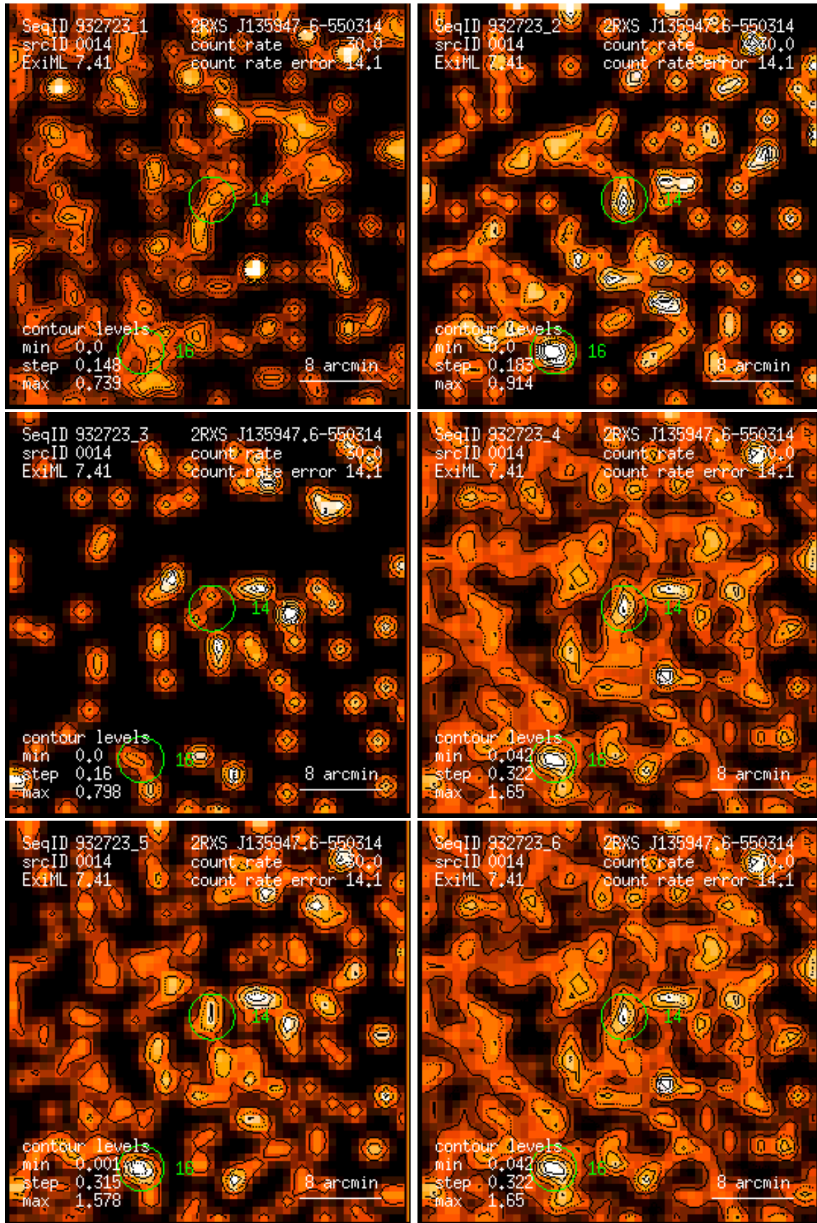
Figure 14: RASS 932723: detection 0014: band rate images, Gaussian filter: (1) PSPC channels 11 – 41, (2) 52 – 90, (3) 91 – 201, (4) 11 – 235, (5) 52 – 201, (6) 11 – 201. Broad band rates in counts/ks. Band rate contour levels in counts/ks/arcmin 2 .
