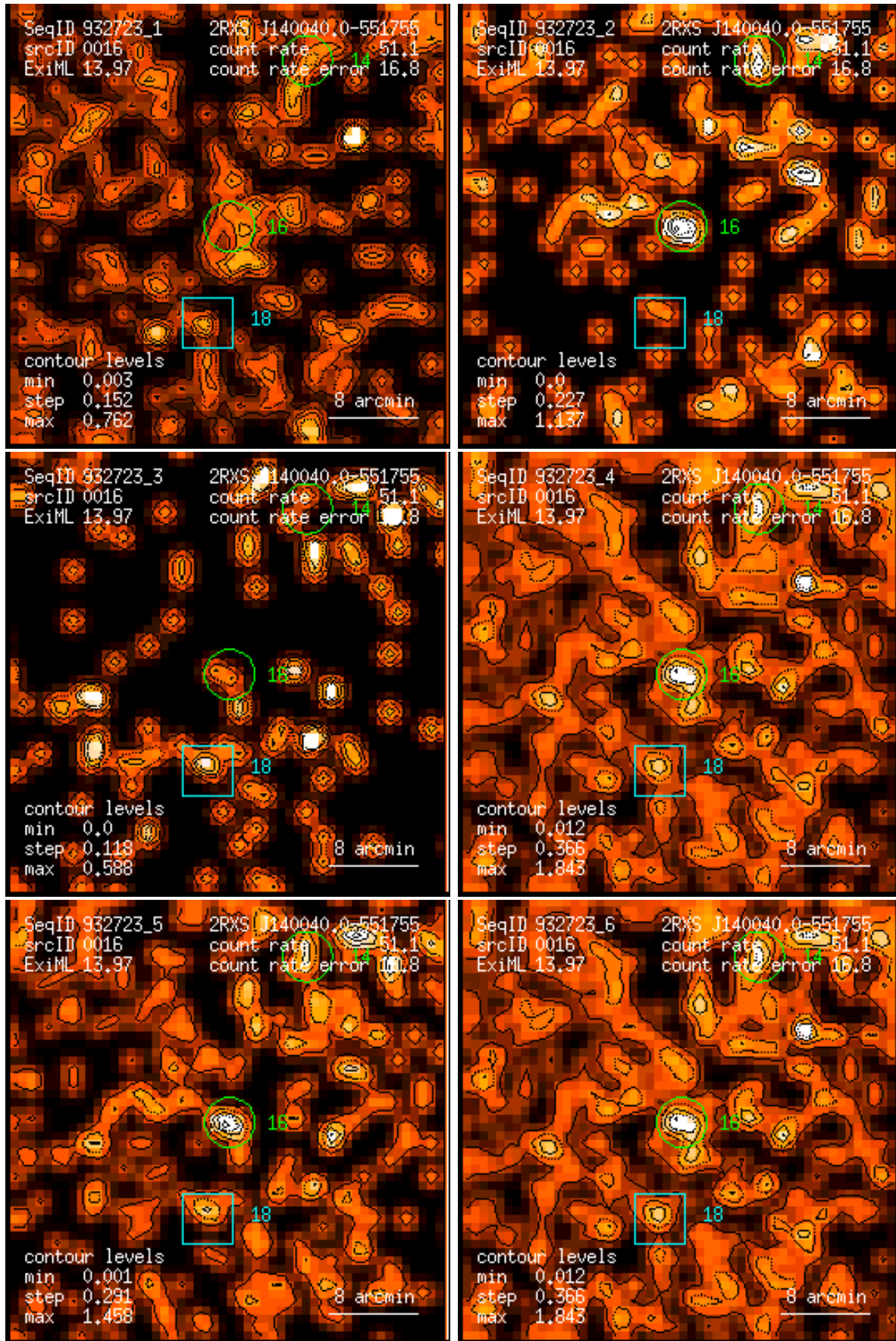
Figure 16: RASS 932723: detection 0016: band rate images, Gaussian filter: (1) PSPC channels 11 – 41, (2) 52 – 90, (3) 91 – 201, (4) 11 – 235, (5) 52 – 201, (6) 11 – 201. Broad band rates in counts/ks. Band rate contour levels in counts/ks/arcmin 2 .
