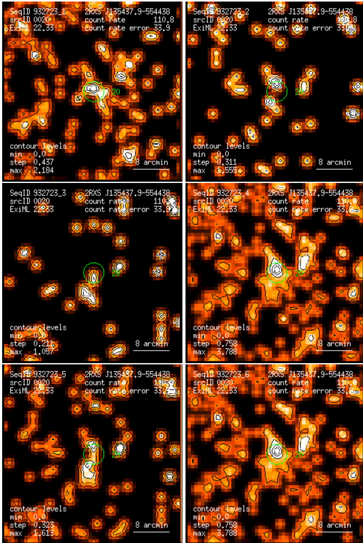
Figure 20: RASS 932723: detection 0020: band rate images, Gaussian filter: (1) PSPC channels 11 – 41, (2) 52 – 90, (3) 91 – 201, (4) 11 – 235, (5) 52 – 201, (6) 11 – 201. Broad band rates in counts/ks. Band rate contour levels in counts/ks/arcmin 2 .
