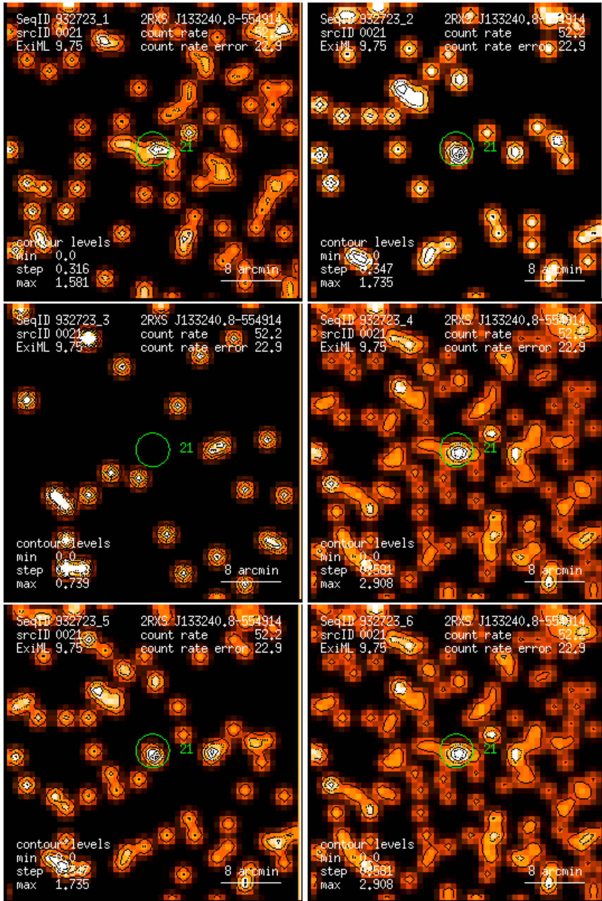
Figure 21: RASS 932723: detection 0021: band rate images, Gaussian filter: (1) PSPC channels 11 – 41, (2) 52 – 90, (3) 91 – 201, (4) 11 – 235, (5) 52 – 201, (6) 11 – 201. Broad band rates in counts/ks. Band rate contour levels in counts/ks/arcmin 2 .
