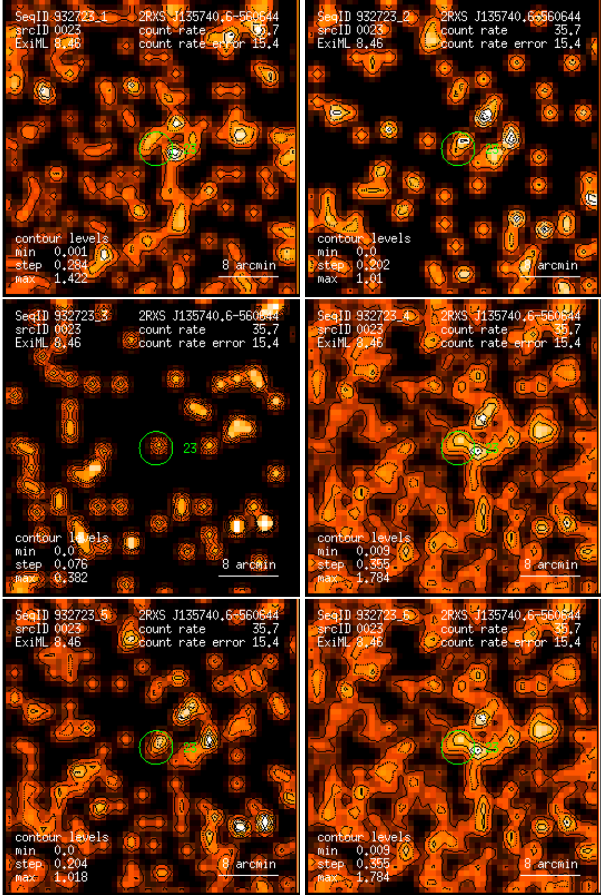
Figure 23: RASS 932723: detection 0023: band rate images, Gaussian filter: (1) PSPC channels 11 – 41, (2) 52 – 90, (3) 91 – 201, (4) 11 – 235, (5) 52 – 201, (6) 11 – 201. Broad band rates in counts/ks. Band rate contour levels in counts/ks/arcmin 2 .
