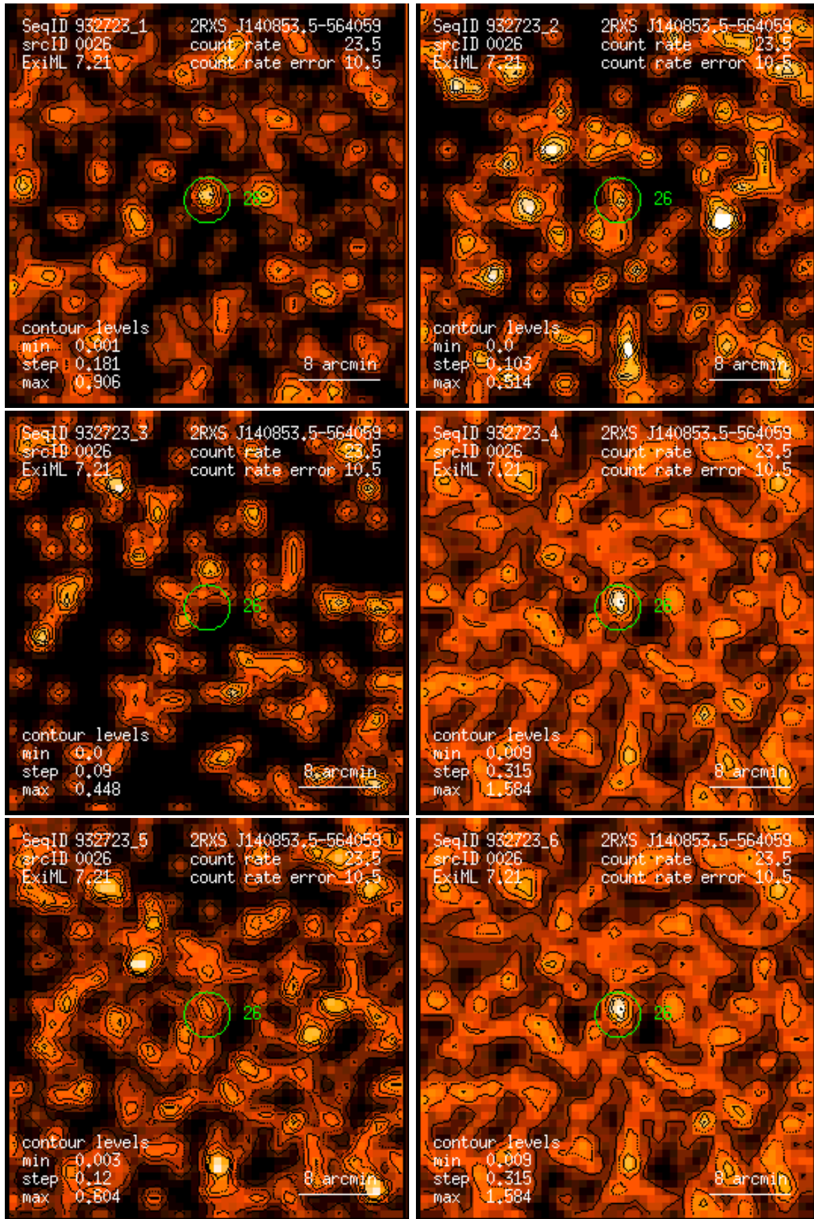
Figure 26: RASS 932723: detection 0026: band rate images, Gaussian filter: (1) PSPC channels 11 – 41, (2) 52 – 90, (3) 91 – 201, (4) 11 – 235, (5) 52 – 201, (6) 11 – 201. Broad band rates in counts/ks. Band rate contour levels in counts/ks/arcmin 2 .
