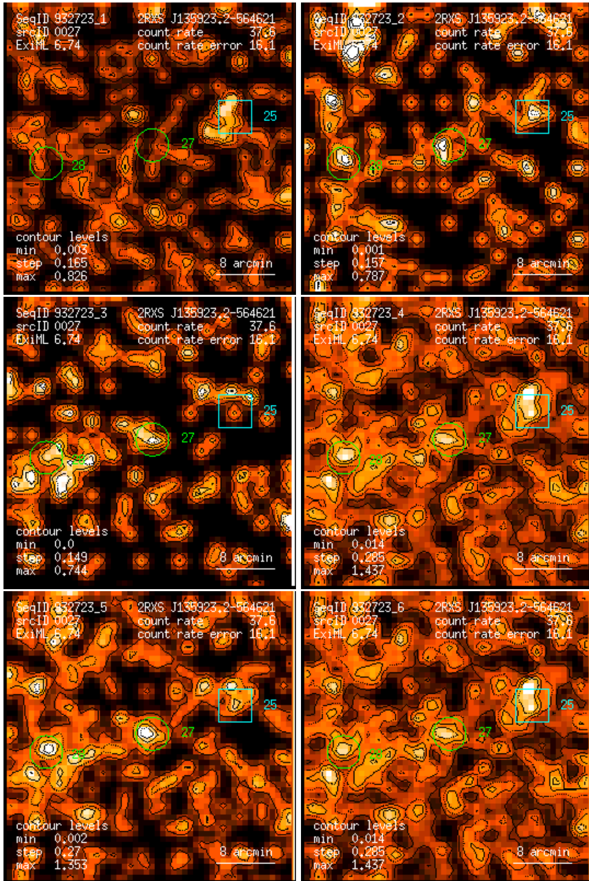
Figure 27: RASS 932723: detection 0027: band rate images, Gaussian filter: (1) PSPC channels 11 – 41, (2) 52 – 90, (3) 91 – 201, (4) 11 – 235, (5) 52 – 201, (6) 11 – 201. Broad band rates in counts/ks. Band rate contour levels in counts/ks/arcmin 2 .
