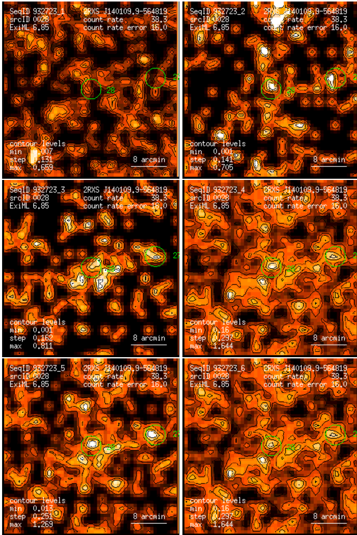
Figure 28: RASS 932723: detection 0028: band rate images, Gaussian filter: (1) PSPC channels 11 – 41, (2) 52 – 90, (3) 91 – 201, (4) 11 – 235, (5) 52 – 201, (6) 11 – 201. Broad band rates in counts/ks. Band rate contour levels in counts/ks/arcmin 2 .
