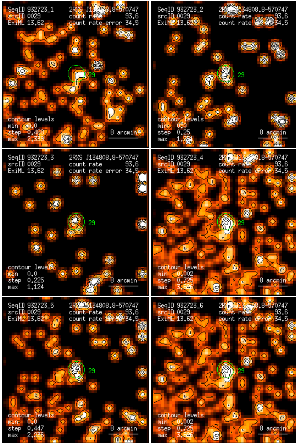
Figure 29: RASS 932723: detection 0029: band rate images, Gaussian filter: (1) PSPC channels 11 – 41, (2) 52 – 90, (3) 91 – 201, (4) 11 – 235, (5) 52 – 201, (6) 11 – 201. Broad band rates in counts/ks. Band rate contour levels in counts/ks/arcmin 2 .
