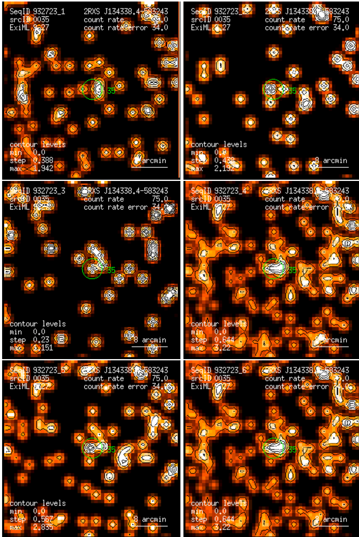
Figure 35: RASS 932723: detection 0035: band rate images, Gaussian filter: (1) PSPC channels 11 – 41, (2) 52 – 90, (3) 91 – 201, (4) 11 – 235, (5) 52 – 201, (6) 11 – 201. Broad band rates in counts/ks. Band rate contour levels in counts/ks/arcmin 2 .
