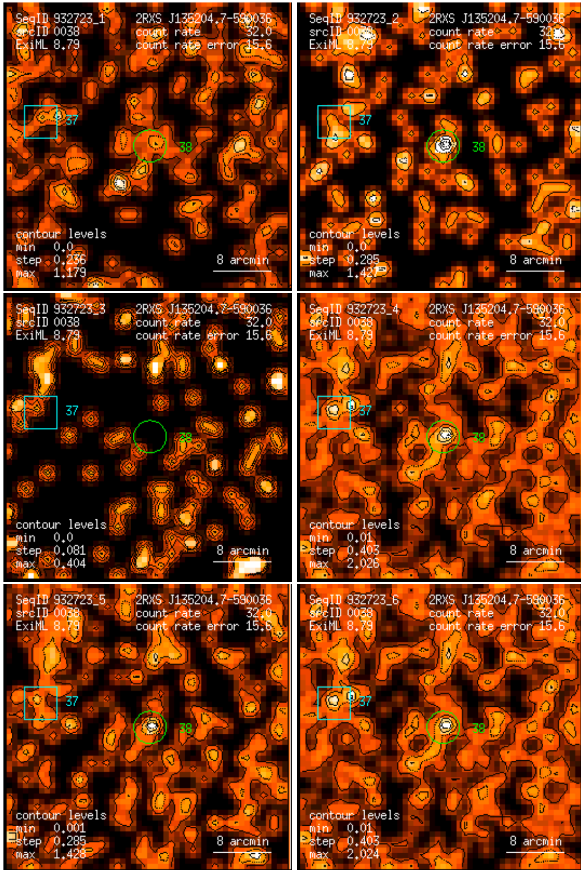
Figure 38: RASS 932723: detection 0038: band rate images, Gaussian filter: (1) PSPC channels 11 – 41, (2) 52 – 90, (3) 91 – 201, (4) 11 – 235, (5) 52 – 201, (6) 11 – 201. Broad band rates in counts/ks. Band rate contour levels in counts/ks/arcmin 2 .
