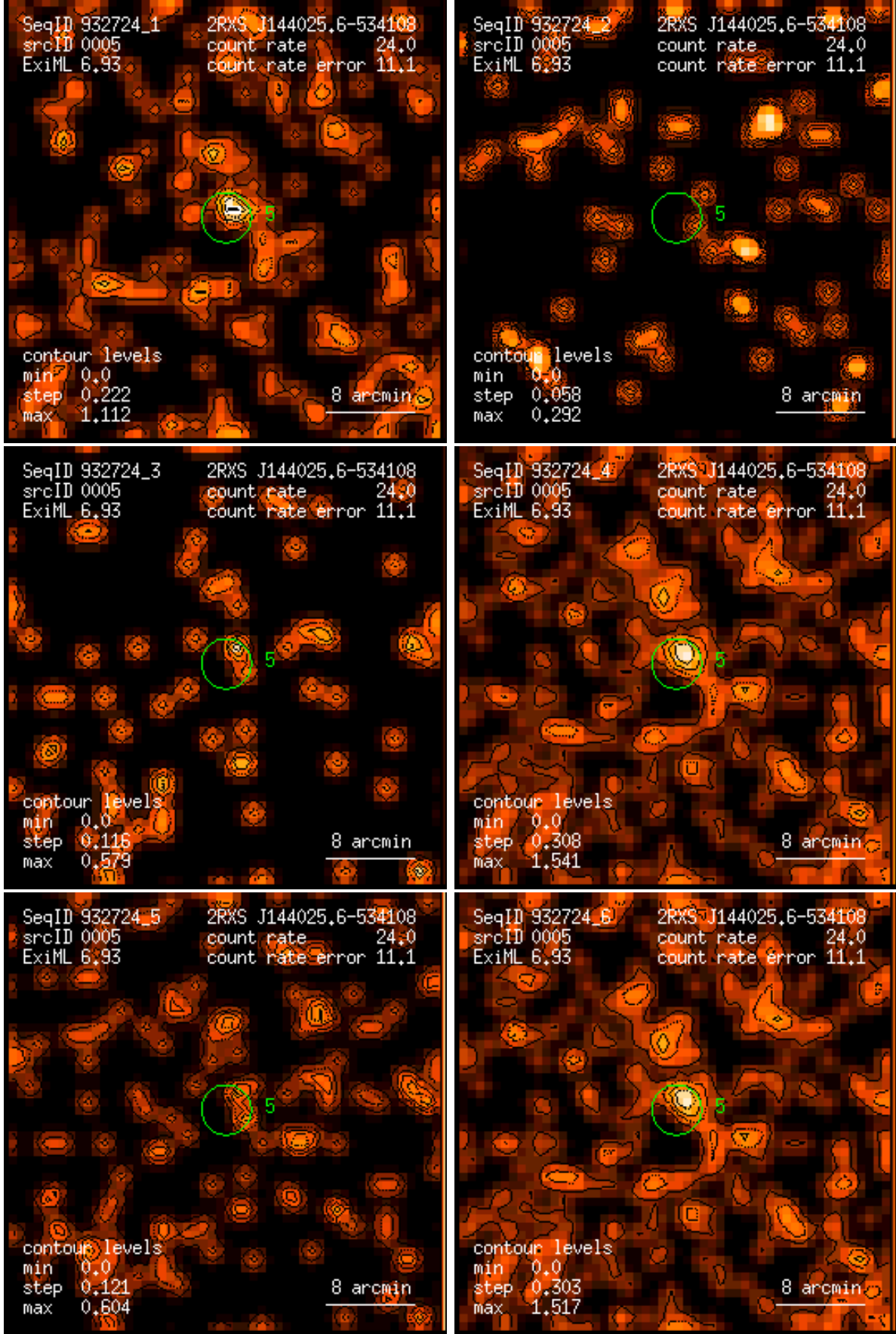
Figure 5: RASS 932724: detection 0005: band rate images, Gaussian filter: (1) PSPC channels 11 – 41, (2) 52 – 90, (3) 91 – 201, (4) 11 – 235, (5) 52 – 201, (6) 11 – 201. Broad band rates in counts/ks. Band rate contour levels in counts/ks/arcmin 2 .
