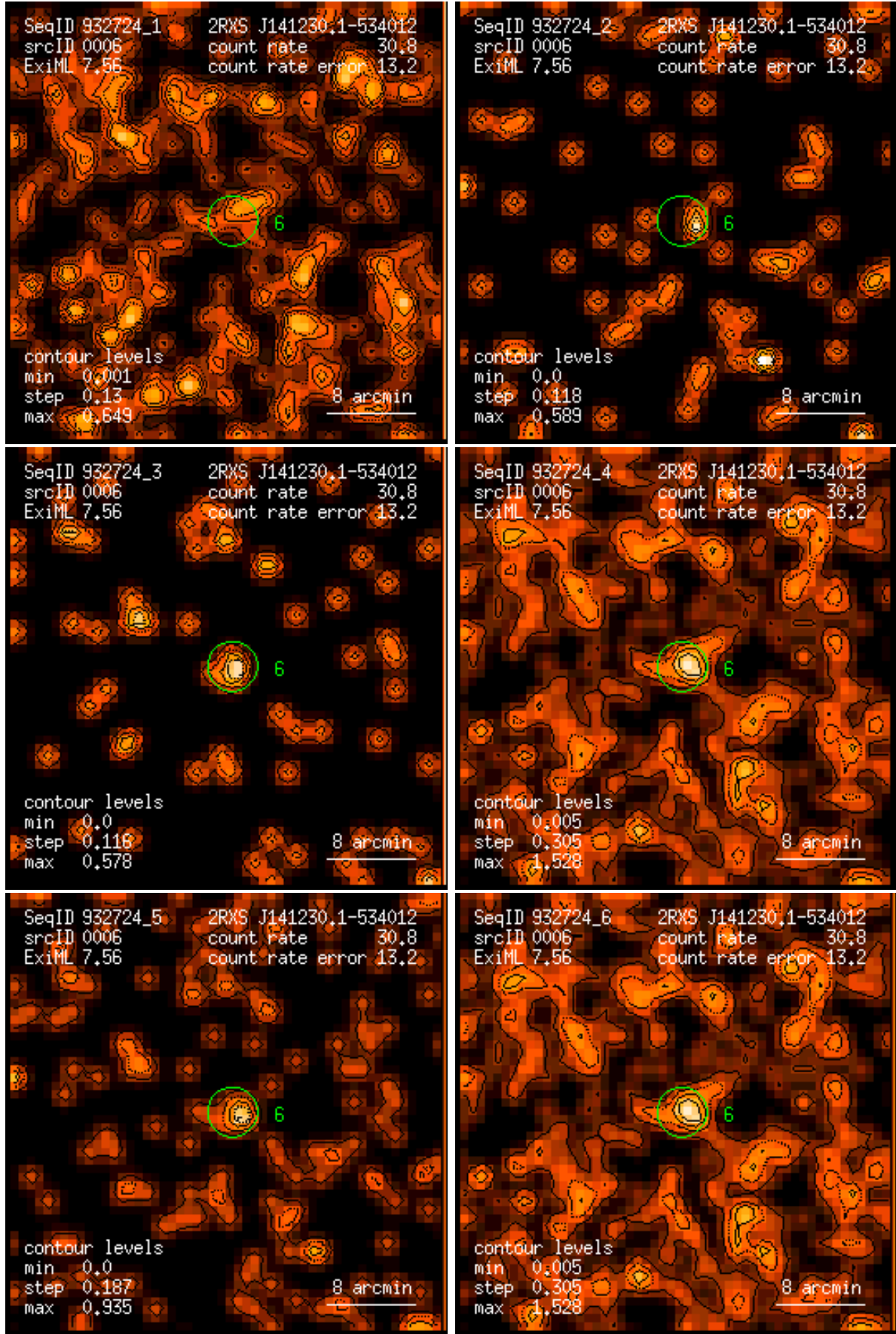
Figure 6: RASS 932724: detection 0006: band rate images, Gaussian filter: (1) PSPC channels 11 – 41, (2) 52 – 90, (3) 91 – 201, (4) 11 – 235, (5) 52 – 201, (6) 11 – 201. Broad band rates in counts/ks. Band rate contour levels in counts/ks/arcmin 2 .
