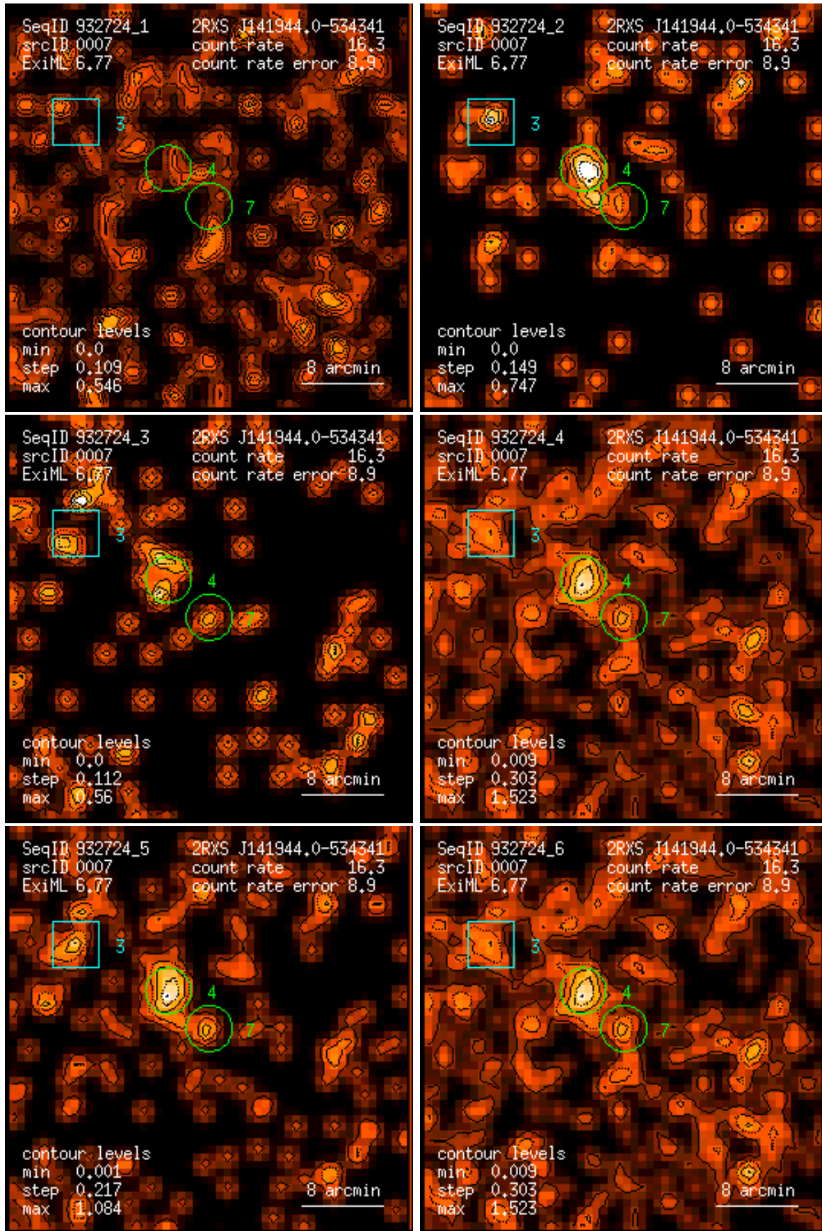
Figure 7: RASS 932724: detection 0007: band rate images, Gaussian filter: (1) PSPC channels 11 – 41, (2) 52 – 90, (3) 91 – 201, (4) 11 – 235, (5) 52 – 201, (6) 11 – 201. Broad band rates in counts/ks. Band rate contour levels in counts/ks/arcmin 2 .
