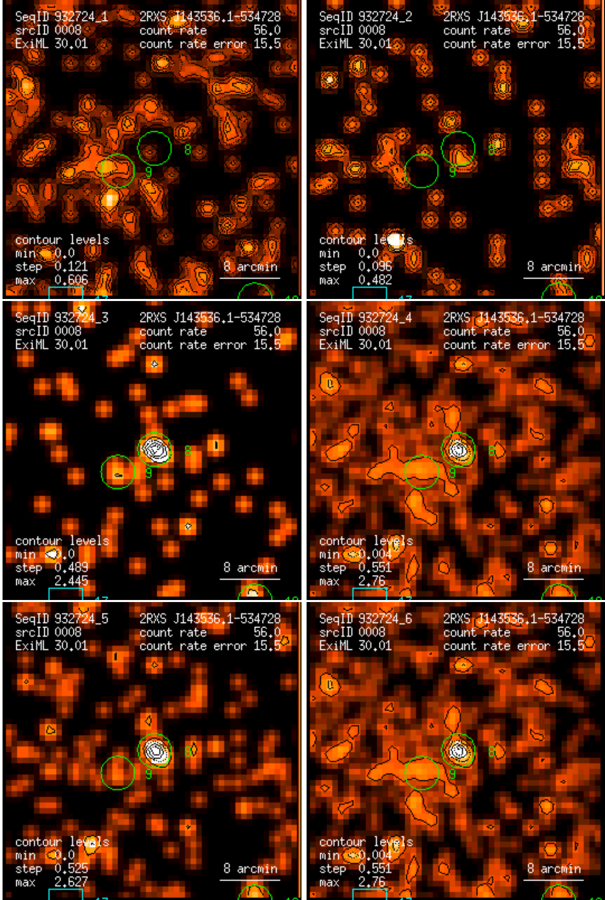
Figure 8: RASS 932724: detection 0008: band rate images, Gaussian filter: (1) PSPC channels 11 – 41, (2) 52 – 90, (3) 91 – 201, (4) 11 – 235, (5) 52 – 201, (6) 11 – 201. Broad band rates in counts/ks. Band rate contour levels in counts/ks/arcmin 2 .
