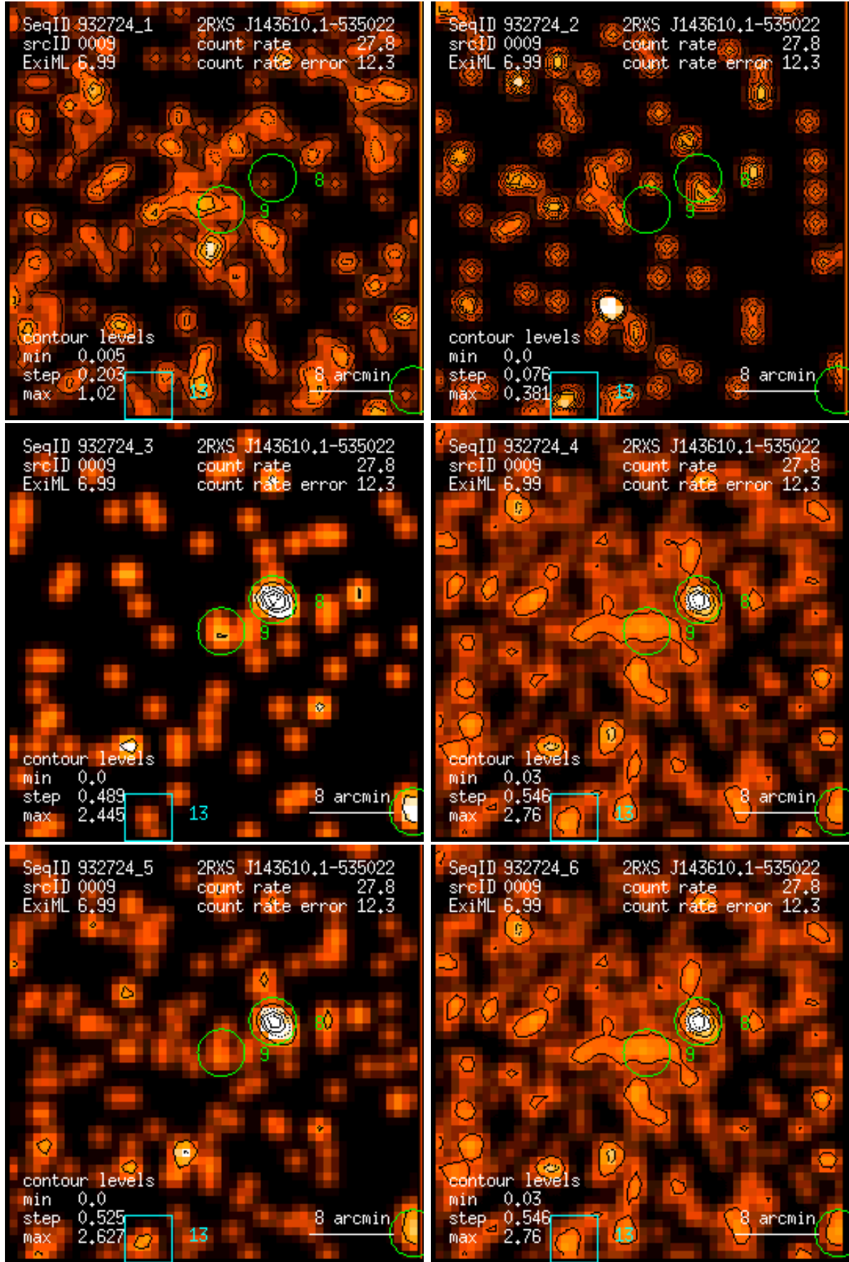
Figure 9: RASS 932724: detection 0009: band rate images, Gaussian filter: (1) PSPC channels 11 – 41, (2) 52 – 90, (3) 91 – 201, (4) 11 – 235, (5) 52 – 201, (6) 11 – 201. Broad band rates in counts/ks. Band rate contour levels in counts/ks/arcmin 2 .
