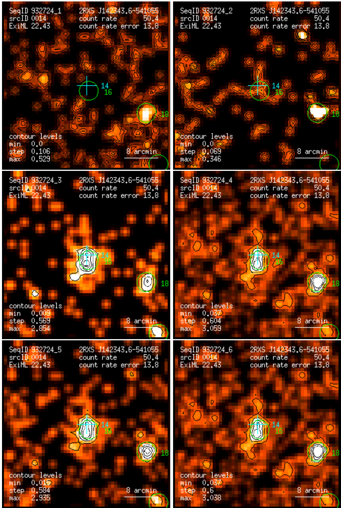
Figure 14: RASS 932724: detection 0014: band rate images, Gaussian filter: (1) PSPC channels 11 – 41, (2) 52 – 90, (3) 91 – 201, (4) 11 – 235, (5) 52 – 201, (6) 11 – 201. Broad band rates in counts/ks. Band rate contour levels in counts/ks/arcmin 2 .
