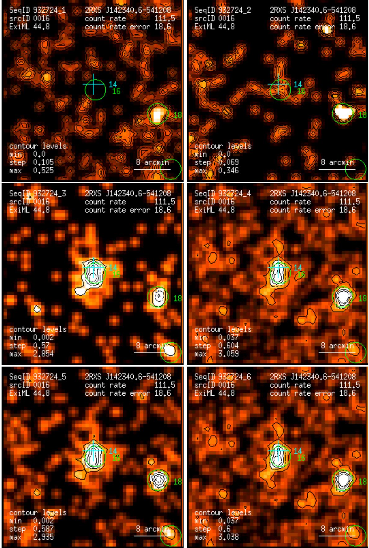
Figure 16: RASS 932724: detection 0016: band rate images, Gaussian filter: (1) PSPC channels 11 – 41, (2) 52 – 90, (3) 91 – 201, (4) 11 – 235, (5) 52 – 201, (6) 11 – 201. Broad band rates in counts/ks. Band rate contour levels in counts/ks/arcmin 2 .
