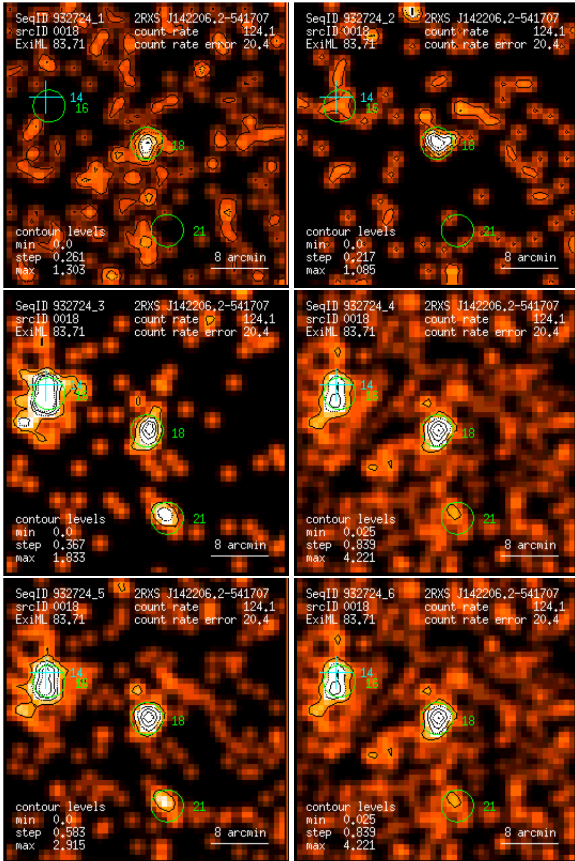
Figure 18: RASS 932724: detection 0018: band rate images, Gaussian filter: (1) PSPC channels 11 – 41, (2) 52 – 90, (3) 91 – 201, (4) 11 – 235, (5) 52 – 201, (6) 11 – 201. Broad band rates in counts/ks. Band rate contour levels in counts/ks/arcmin 2 .
