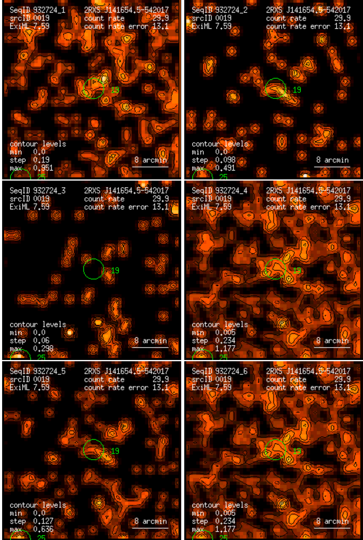
Figure 19: RASS 932724: detection 0019: band rate images, Gaussian filter: (1) PSPC channels 11 – 41, (2) 52 – 90, (3) 91 – 201, (4) 11 – 235, (5) 52 – 201, (6) 11 – 201. Broad band rates in counts/ks. Band rate contour levels in counts/ks/arcmin 2 .
