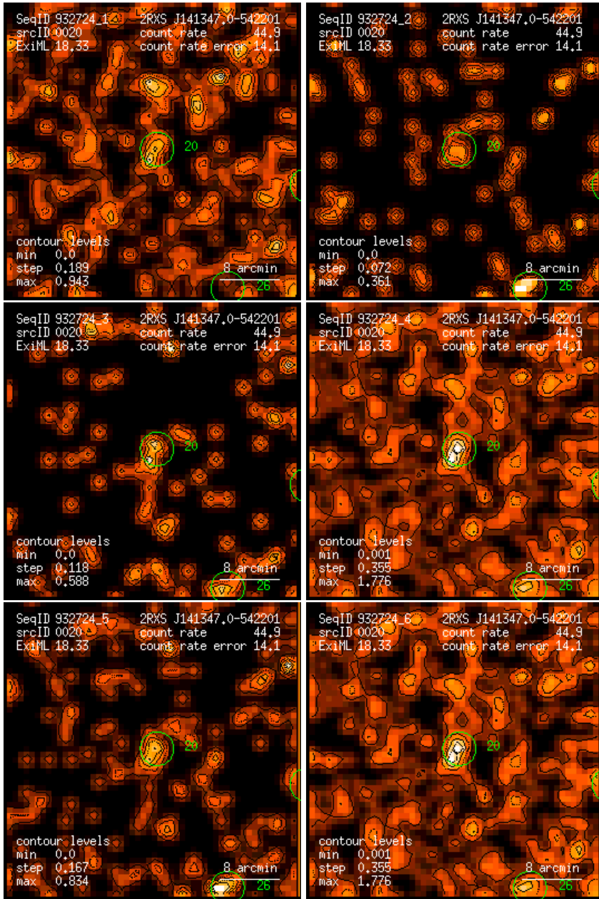
Figure 20: RASS 932724: detection 0020: band rate images, Gaussian filter: (1) PSPC channels 11 – 41, (2) 52 – 90, (3) 91 – 201, (4) 11 – 235, (5) 52 – 201, (6) 11 – 201. Broad band rates in counts/ks. Band rate contour levels in counts/ks/arcmin 2 .
