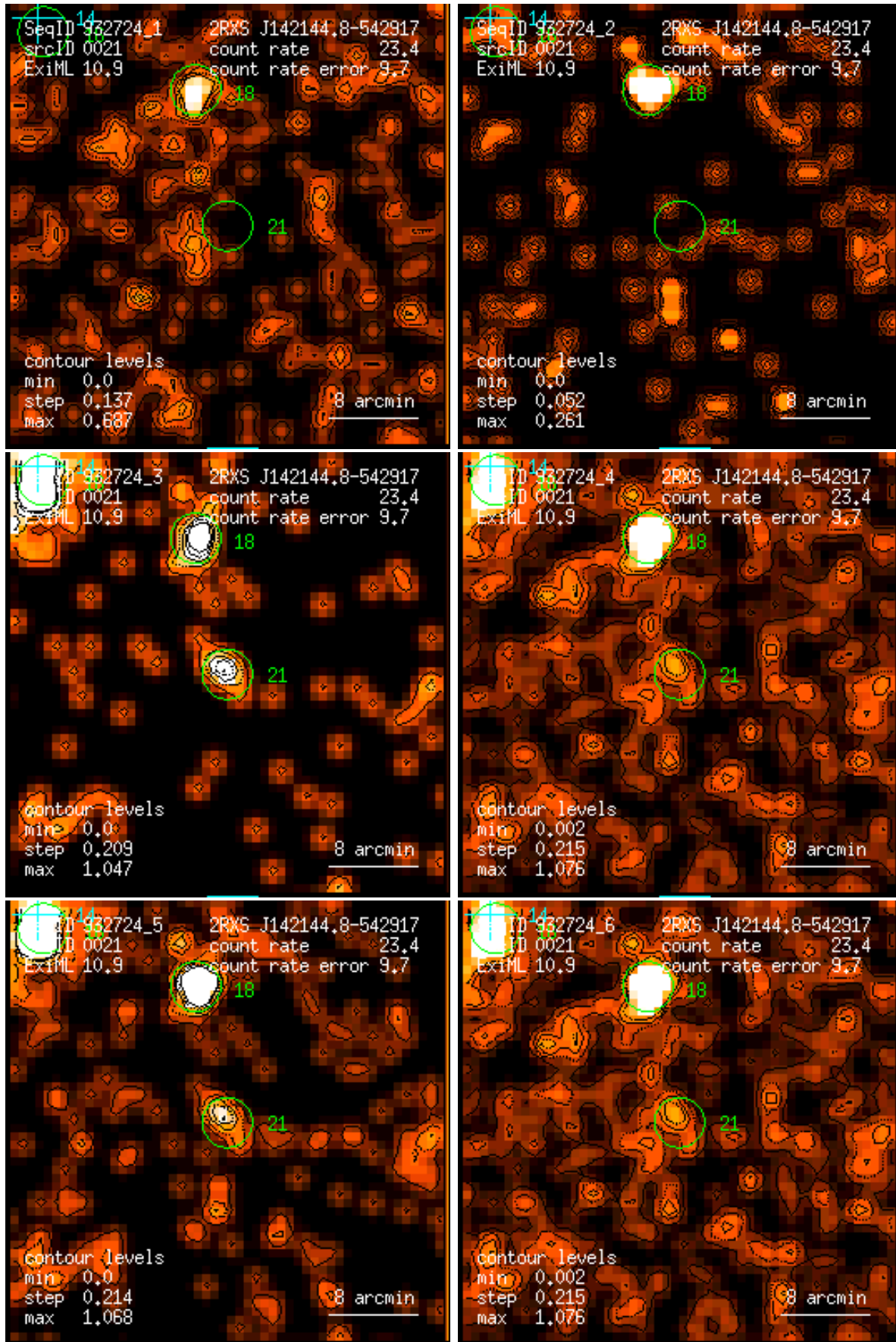
Figure 21: RASS 932724: detection 0021: band rate images, Gaussian filter: (1) PSPC channels 11 – 41, (2) 52 – 90, (3) 91 – 201, (4) 11 – 235, (5) 52 – 201, (6) 11 – 201. Broad band rates in counts/ks. Band rate contour levels in counts/ks/arcmin 2 .
