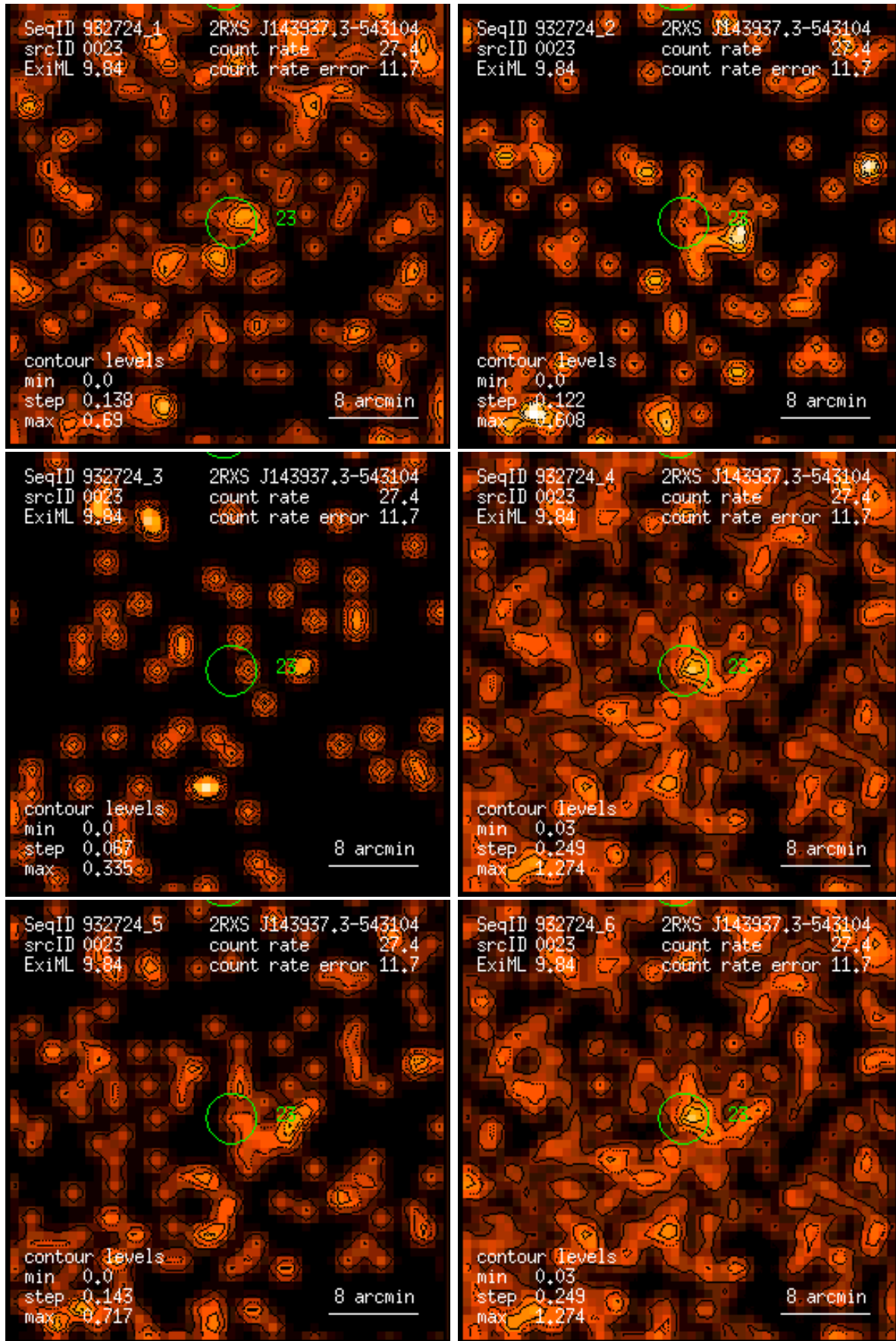
Figure 23: RASS 932724: detection 0023: band rate images, Gaussian filter: (1) PSPC channels 11 – 41, (2) 52 – 90, (3) 91 – 201, (4) 11 – 235, (5) 52 – 201, (6) 11 – 201. Broad band rates in counts/ks. Band rate contour levels in counts/ks/arcmin 2 .
