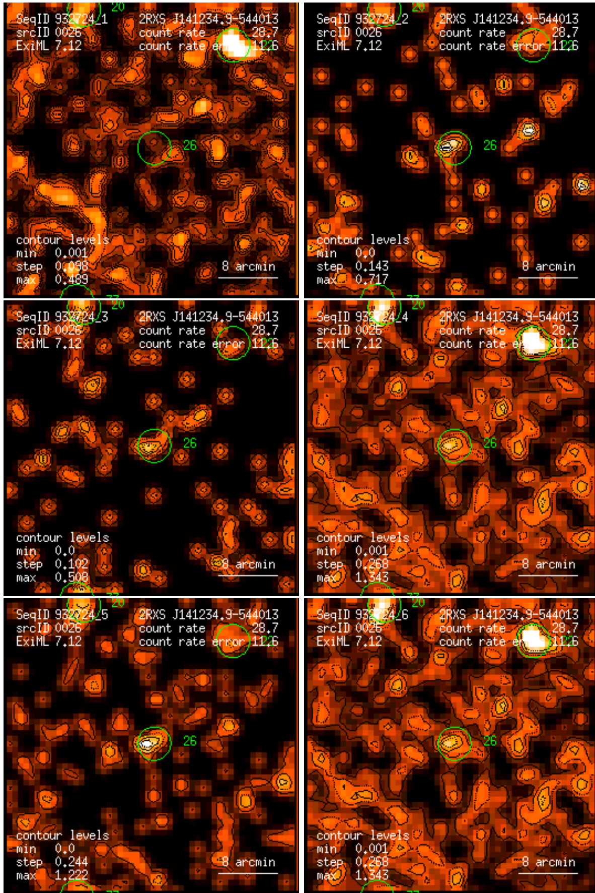
Figure 26: RASS 932724: detection 0026: band rate images, Gaussian filter: (1) PSPC channels 11 – 41, (2) 52 – 90, (3) 91 – 201, (4) 11 – 235, (5) 52 – 201, (6) 11 – 201. Broad band rates in counts/ks. Band rate contour levels in counts/ks/arcmin 2 .
