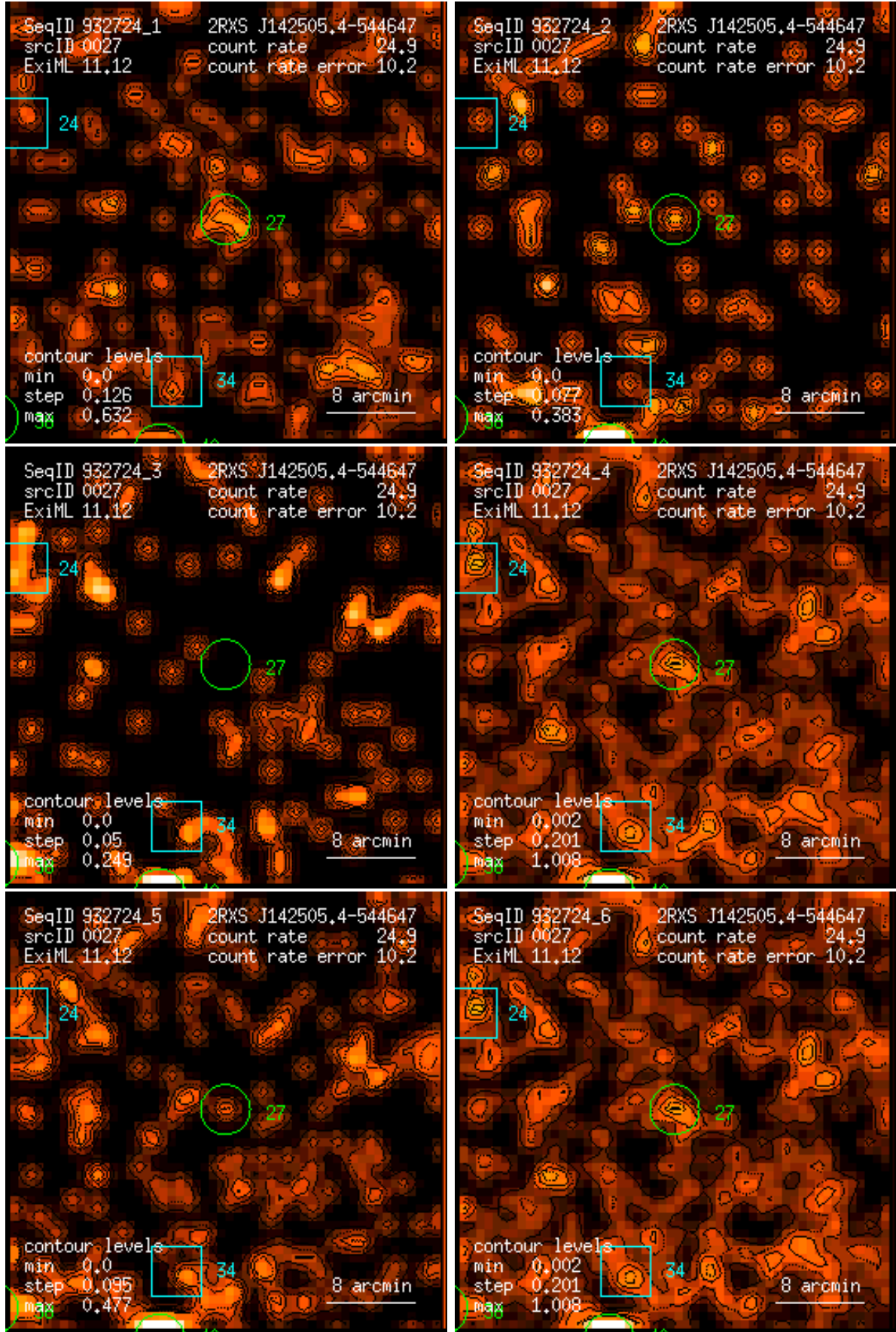
Figure 27: RASS 932724: detection 0027: band rate images, Gaussian filter: (1) PSPC channels 11 – 41, (2) 52 – 90, (3) 91 – 201, (4) 11 – 235, (5) 52 – 201, (6) 11 – 201. Broad band rates in counts/ks. Band rate contour levels in counts/ks/arcmin 2 .
