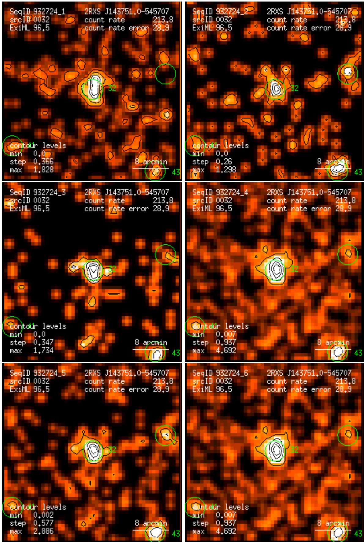
Figure 32: RASS 932724: detection 0032: band rate images, Gaussian filter: (1) PSPC channels 11 – 41, (2) 52 – 90, (3) 91 – 201, (4) 11 – 235, (5) 52 – 201, (6) 11 – 201. Broad band rates in counts/ks. Band rate contour levels in counts/ks/arcmin 2 .
