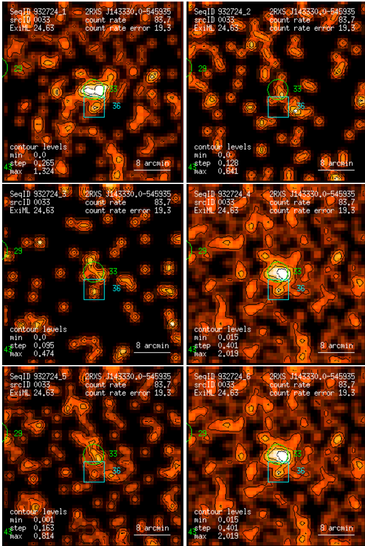
Figure 33: RASS 932724: detection 0033: band rate images, Gaussian filter: (1) PSPC channels 11 – 41, (2) 52 – 90, (3) 91 – 201, (4) 11 – 235, (5) 52 – 201, (6) 11 – 201. Broad band rates in counts/ks. Band rate contour levels in counts/ks/arcmin 2 .
