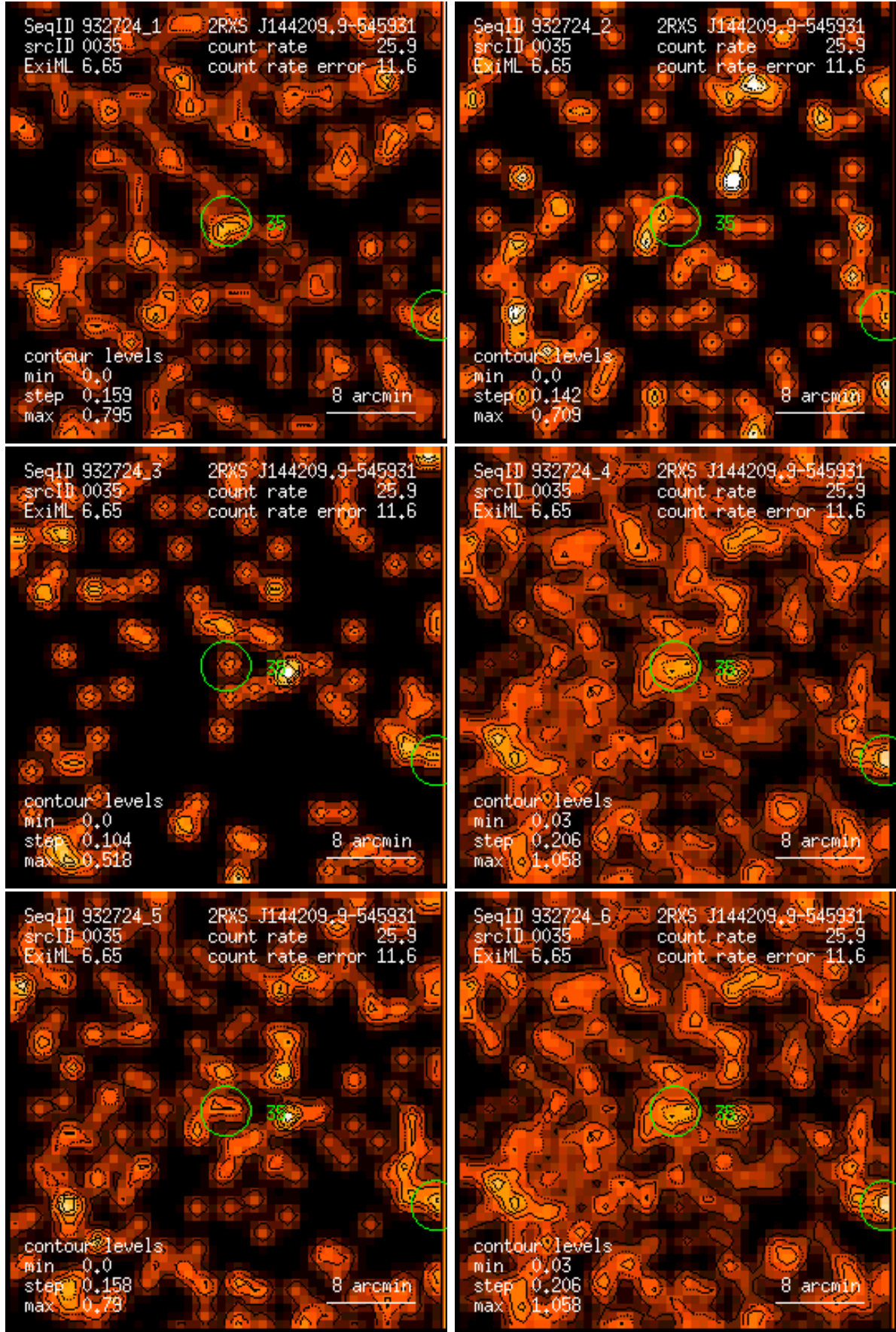
Figure 35: RASS 932724: detection 0035: band rate images, Gaussian filter: (1) PSPC channels 11 – 41, (2) 52 – 90, (3) 91 – 201, (4) 11 – 235, (5) 52 – 201, (6) 11 – 201. Broad band rates in counts/ks. Band rate contour levels in counts/ks/arcmin 2 .
