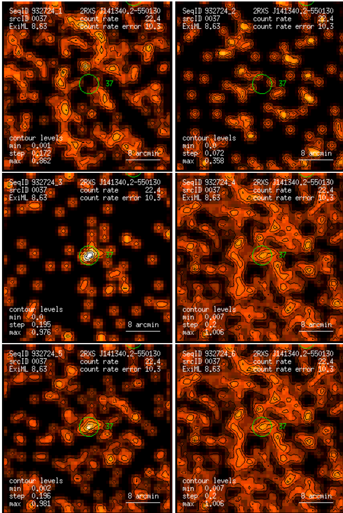
Figure 37: RASS 932724: detection 0037: band rate images, Gaussian filter: (1) PSPC channels 11 – 41, (2) 52 – 90, (3) 91 – 201, (4) 11 – 235, (5) 52 – 201, (6) 11 – 201. Broad band rates in counts/ks. Band rate contour levels in counts/ks/arcmin 2 .
