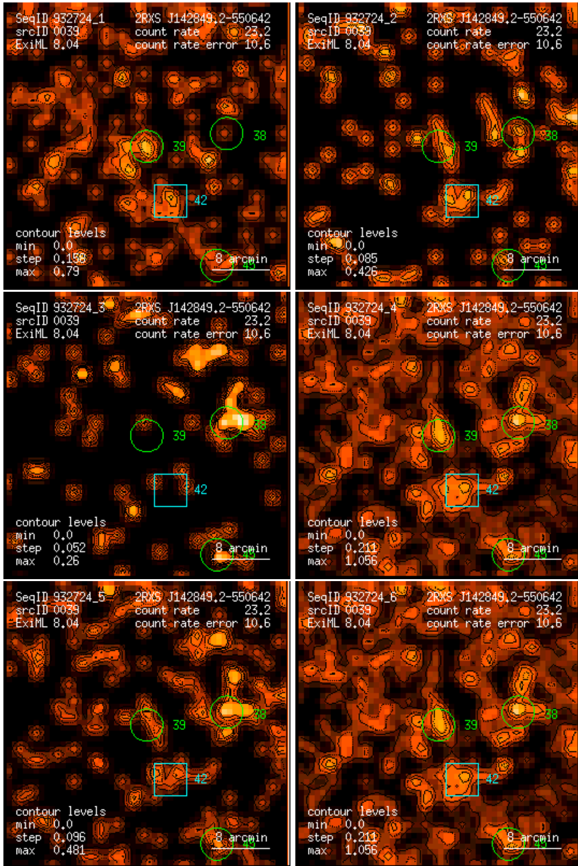
Figure 39: RASS 932724: detection 0039: band rate images, Gaussian filter: (1) PSPP channels 11 – 41, (2) 52 – 90, (3) 91 – 201, (4) 11 – 235, (5) 52 – 201, (6) 11 – 201. Broad band rates in counts/ks. Band rate contour levels in counts/ks/arcmin 2 .
