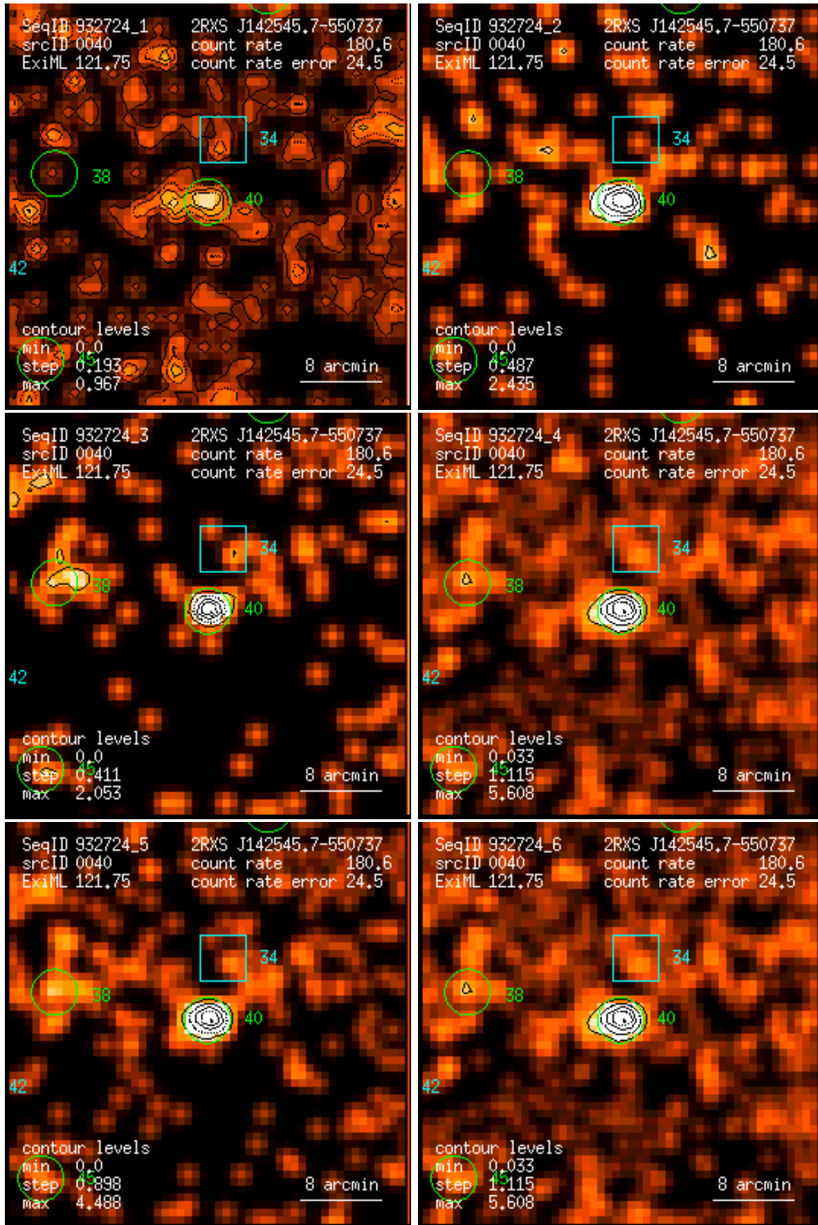
Figure 40: RASS 932724: detection 0040: band rate images, Gaussian filter: (1) PSPC channels 11 – 41, (2) 52 – 90, (3) 91 – 201, (4) 11 – 235, (5) 52 – 201, (6) 11 – 201. Broad band rates in counts/ks. Band rate contour levels in counts/ks/arcmin 2 .
