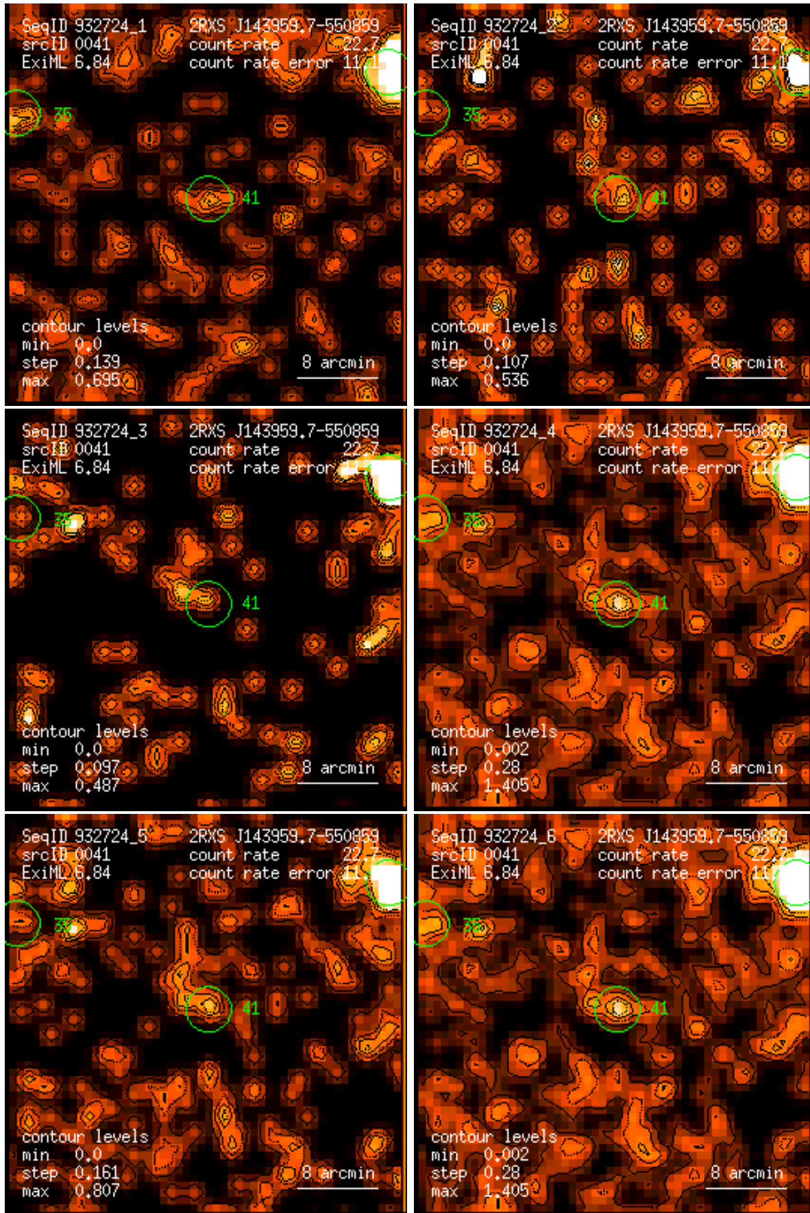
Figure 41: RASS 932724: detection 0041: band rate images, Gaussian filter: (1) PSPC channels 11 – 41, (2) 52 – 90, (3) 91 – 201, (4) 11 – 235, (5) 52 – 201, (6) 11 – 201. Broad band rates in counts/ks. Band rate contour levels in counts/ks/arcmin 2 .
