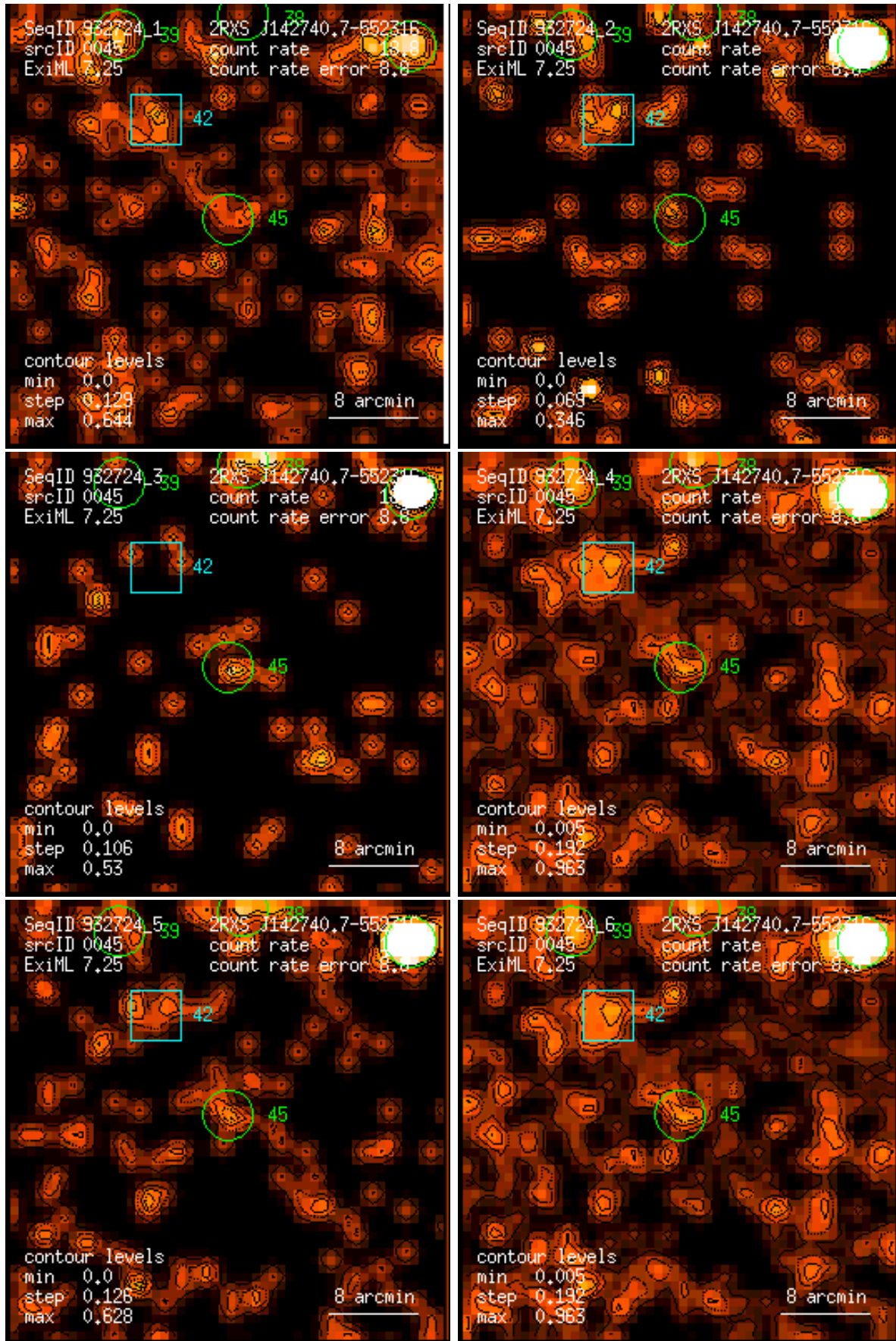
Figure 45: RASS 932724: detection 0045: band rate images, Gaussian filter: (1) PSPC channels 11 – 41, (2) 52 – 90, (3) 91 – 201, (4) 11 – 235, (5) 52 – 201, (6) 11 – 201. Broad band rates in counts/ks. Band rate contour levels in counts/ks/arcmin 2 .
