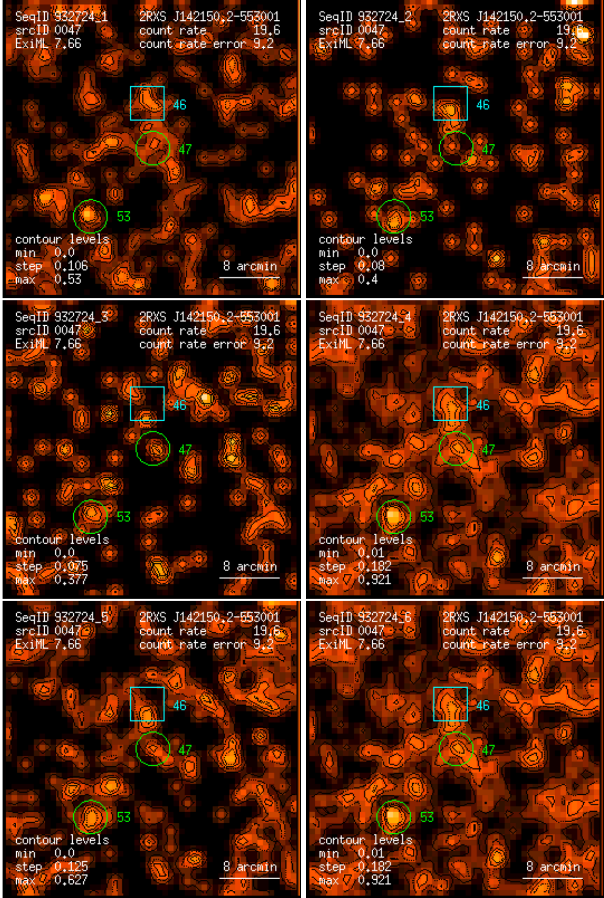
Figure 47: RASS 932724: detection 0047: band rate images, Gaussian filter: (1) PSPC channels 11 – 41, (2) 52 – 90, (3) 91 – 201, (4) 11 – 235, (5) 52 – 201, (6) 11 – 201. Broad band rates in counts/ks. Band rate contour levels in counts/ks/arcmin 2 .
