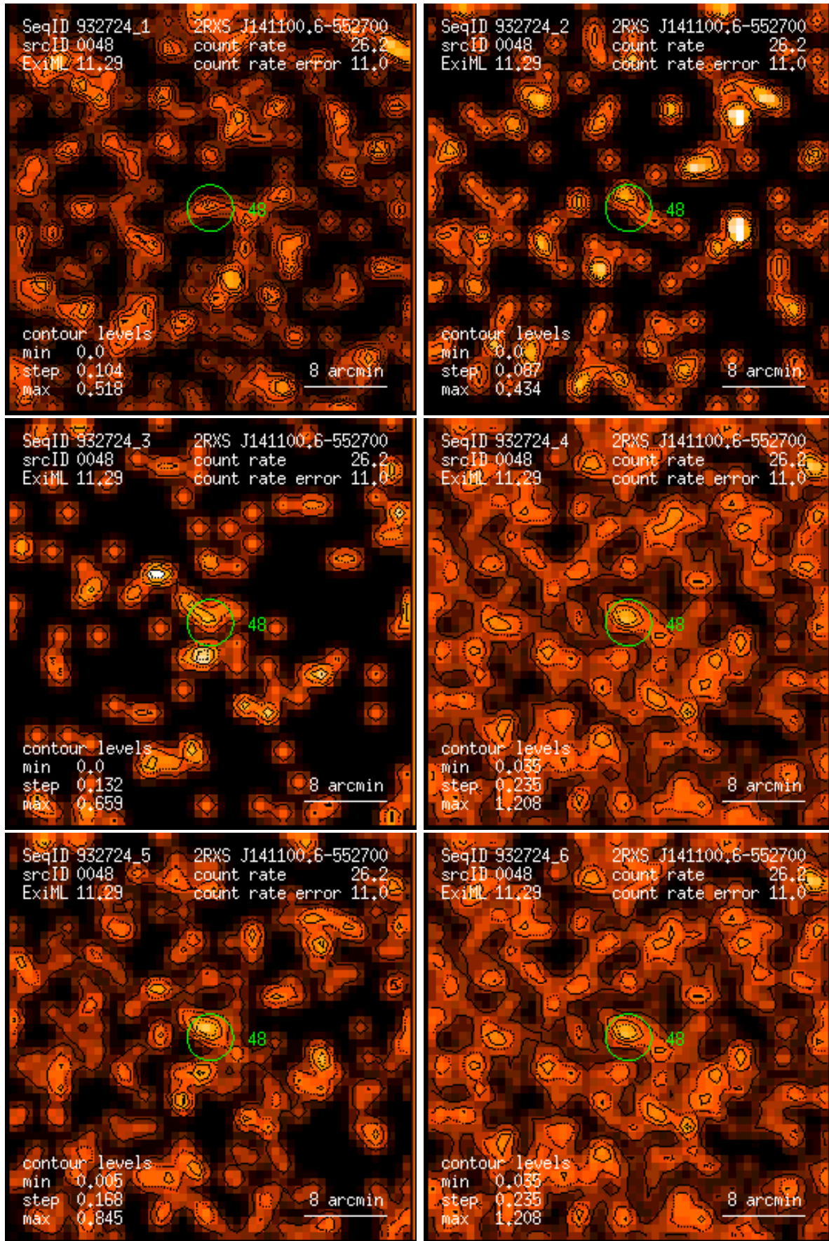
Figure 48: RASS 932724: detection 0048: band rate images, Gaussian filter: (1) PSPC channels 11 – 41, (2) 52 – 90, (3) 91 – 201, (4) 11 – 235, (5) 52 – 201, (6) 11 – 201. Broad band rates in counts/ks. Band rate contour levels in counts/ks/arcmin 2 .
