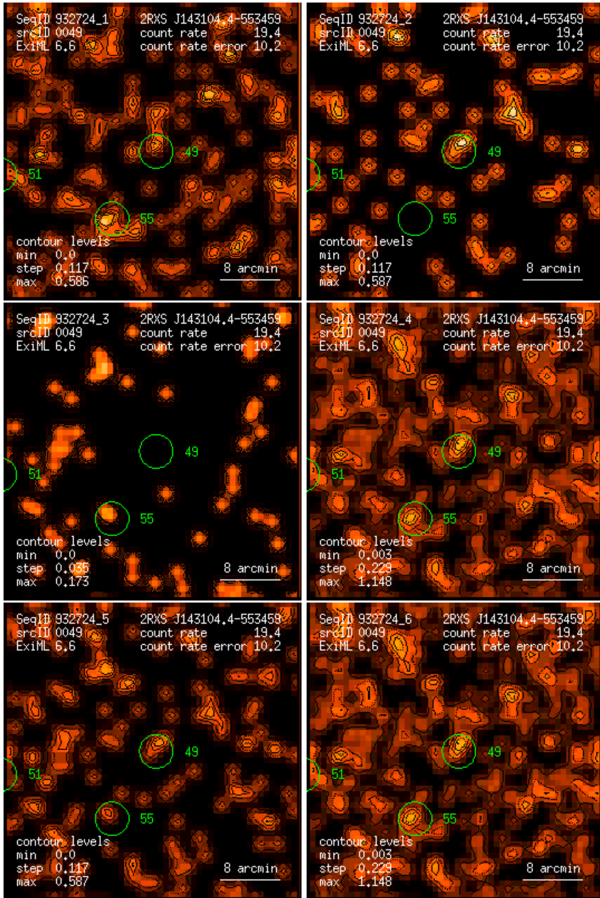
Figure 49: RASS 932724: detection 0049: band rate images, Gaussian filter: (1) PSPC channels 11 – 41, (2) 52 – 90, (3) 91 – 201, (4) 11 – 235, (5) 52 – 201, (6) 11 – 201. Broad band rates in counts/ks. Band rate contour levels in counts/ks/arcmin 2 .
