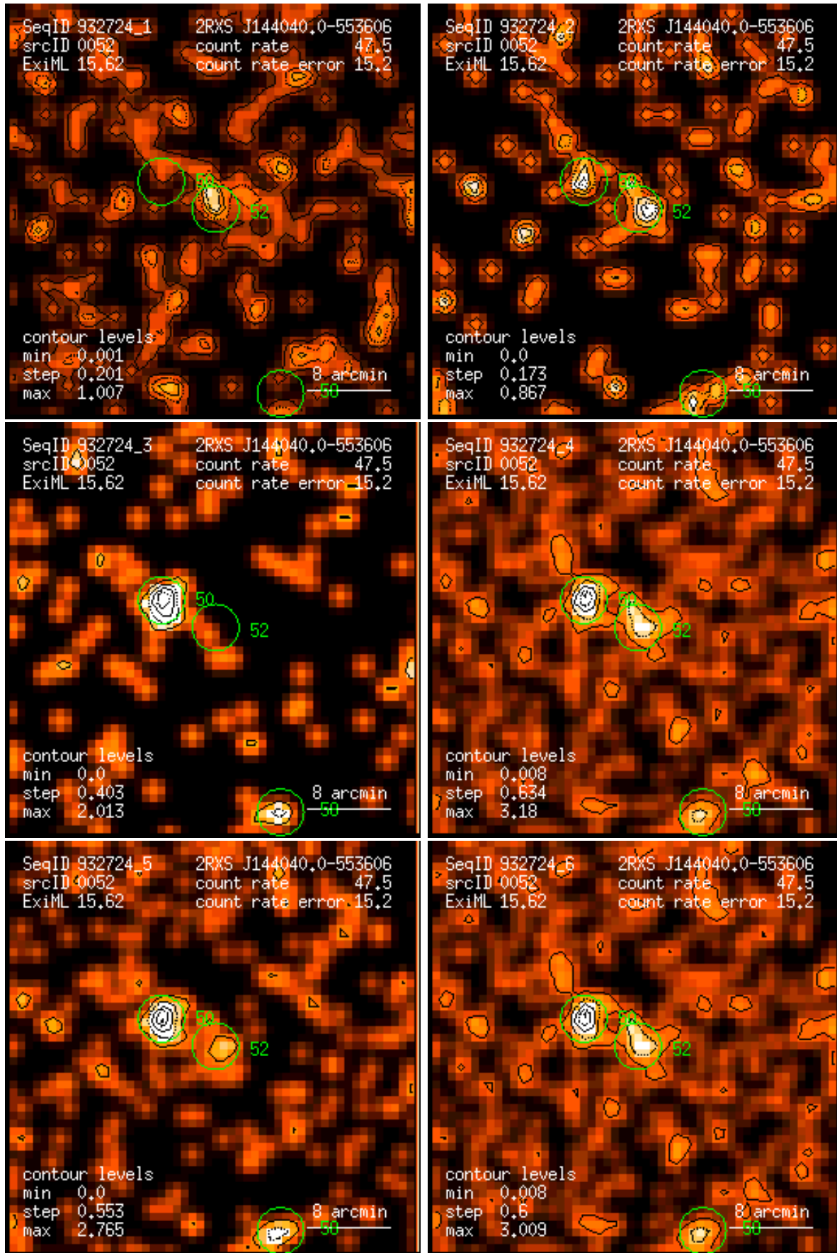
Figure 52: RASS 932724: detection 0052: band rate images, Gaussian filter: (1) PSPC channels 11 – 41, (2) 52 – 90, (3) 91 – 201, (4) 11 – 235, (5) 52 – 201, (6) 11 – 201. Broad band rates in counts/ks. Band rate contour levels in counts/ks/arcmin 2 .
